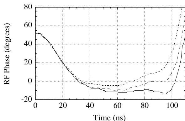
Fig. 2: Phase of beam induced rf measured at different times separated by about 300 hours of processing (first measurement = solid, second = dashed and third = dotted).
