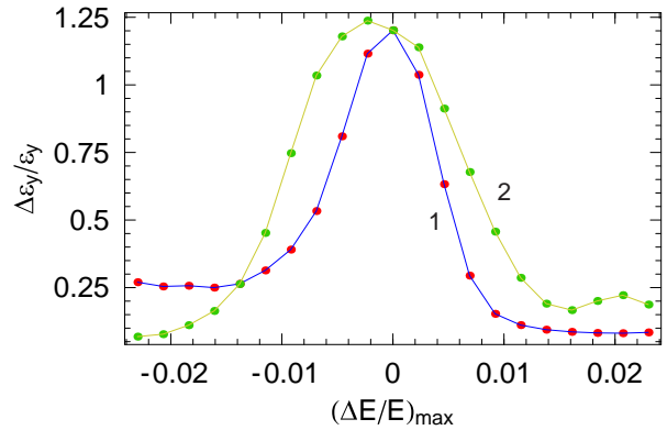
Figure 6: Relative emittance increase as a function of the energy spread for initial train offset of 1 \mu\text{m} . Curve 1 corresponds to a linear variation of the energy, and curve 2 — to exponential function \Delta E_k .
