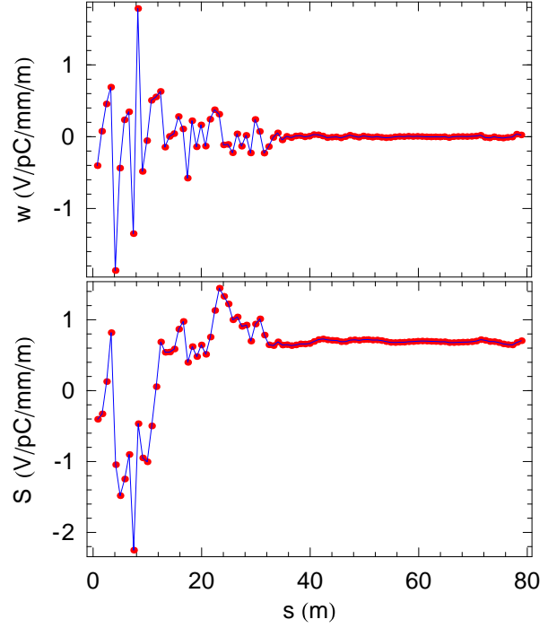
Figure 1: Transverse wake w and the corresponding sum wake S for NLC linac with 3 MHz rms frequency error in the dipole modes. Each point corresponds to a single bunch. The total number of bunches in the train is 95 and the spacing between the bunches is 83 cm.
