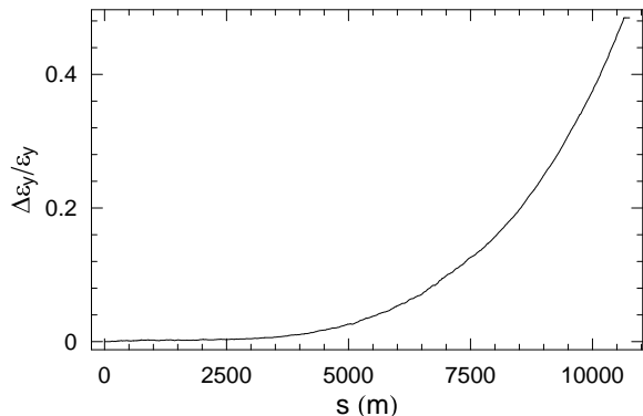
Figure 2: Relative emittance growth along the linac in the train of bunches, for 10 \mu\text{m} rms structure misalignments, when all bunches have the same energy. The bunches are simulated as single particles, so that there is no emittance growth within the bunch.
