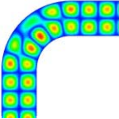
Figure 4: Dual-moded H-plane bend. TE_{10} and TE_{20} pass from input to output unmixed.
