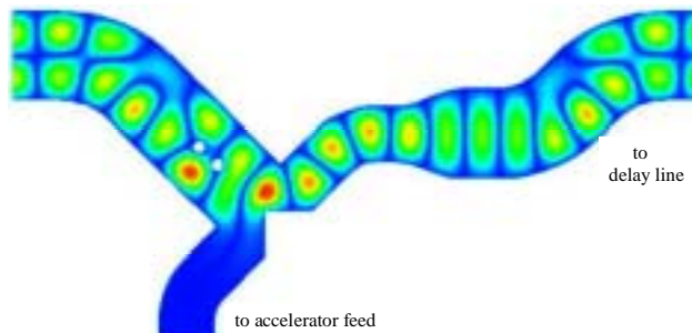
Figure 3: Extractor with jog converter passing TE_{20} . A TE_{10} wave incident from the left would be extracted to the lower port.
