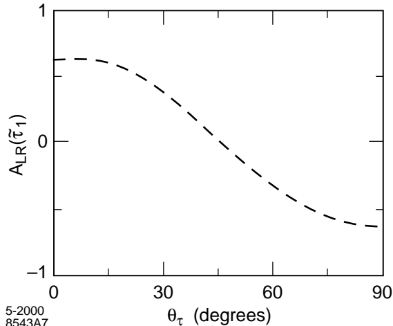
Figure 8: Polarization asymmetry of e^+e^- \rightarrow \tilde{\tau}_1^+\tilde{\tau}_1^- as a function of the stau mixing angle.
