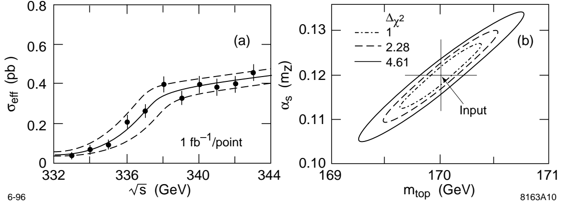
Figure 15: Measurement of the top quark mass from the threshold shape, using a threshold scan with a total data sample of 11 \text{ fb}^{-1} . The effects of beamstrahlung, initial state radiation, and accelerator energy spread are included. A top quark mass of 170 GeV was assumed in this study [89].
