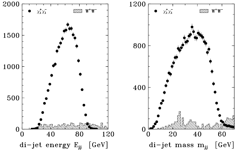
Figure 12: Kinematic distributions from a simulation of chargino pair production and decay with 160 \text{ fb}^{-1} at 320 GeV, from [77]. left: dijet energy distribution; right: dijet mass distribution.
