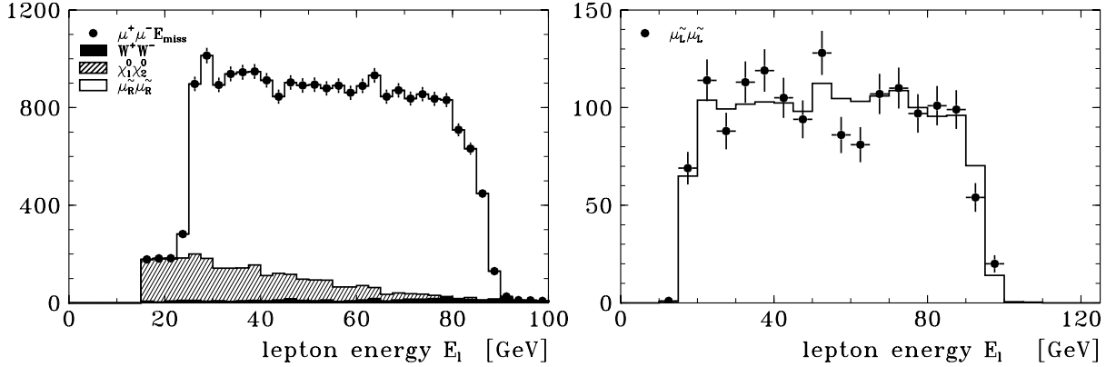
Figure 7: Energy distribution of muons resulting from processes e^+e^- \rightarrow \tilde{\mu}^- \tilde{\mu}^+ , followed by \tilde{\mu} decay, from [77]. left: e^+e^- \rightarrow \tilde{\mu}_R^- \tilde{\mu}_R^+ , for a 160 \text{ fb}^{-1} event sample at 320 GeV; right: e^+e^- \rightarrow \tilde{\mu}_L^- \tilde{\mu}_L^+ , with selection of \tilde{\mu}_L \rightarrow \mu \tilde{\chi}_2^0 , \tilde{\chi}_2^0 \rightarrow \ell^+ \ell^- \tilde{\chi}_1^0 decays on both sides, for a 250 \text{ fb}^{-1} event sample at 500 GeV. The electron beam polarization is used to reduce the background from e^+e^- \rightarrow W^+W^- .
