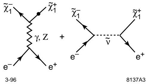
Figure 13: Diagrams contributing to chargino pair production.
