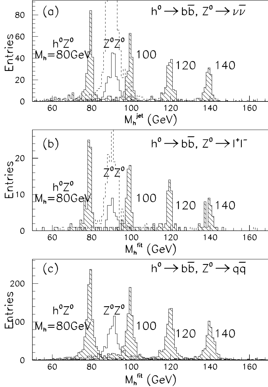
Figure 4: Higgs reconstruction in the process e^+e^- \rightarrow Z^0 h^0 for various Higgs boson masses, using \ell^+\ell^- , \nu\bar{\nu} , and hadronic Z^0 decays, for a 30 \text{ fb}^{-1} event sample at 300 GeV, from [63]. The background is dominated by the process e^+e^- \rightarrow Z^0 Z^0 , which produces the missing-mass peak at m_Z . The unshaded solid histogram gives the background if a b -tag is applied to the Higgs candidate. The dashed histograms in (a) and (b) show the background with no b -tag.
