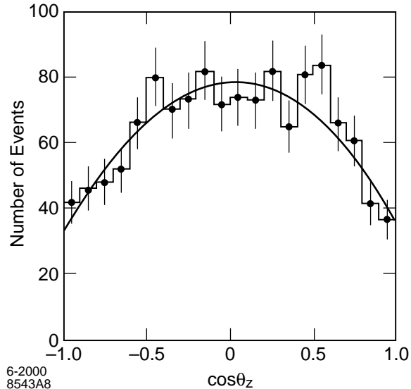
Figure 6: Angular distribution of the Z boson in e^+e^- \rightarrow Z^0 h^0 , as reconstructed from a 50 \text{ fb}^{-1} event sample at 300 GeV, from [69].
