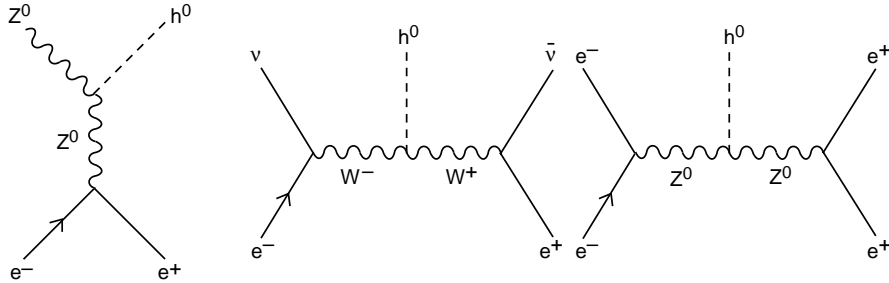
Figure 3: Processes for production of the Higgs boson at an e^+e^- linear collider.
