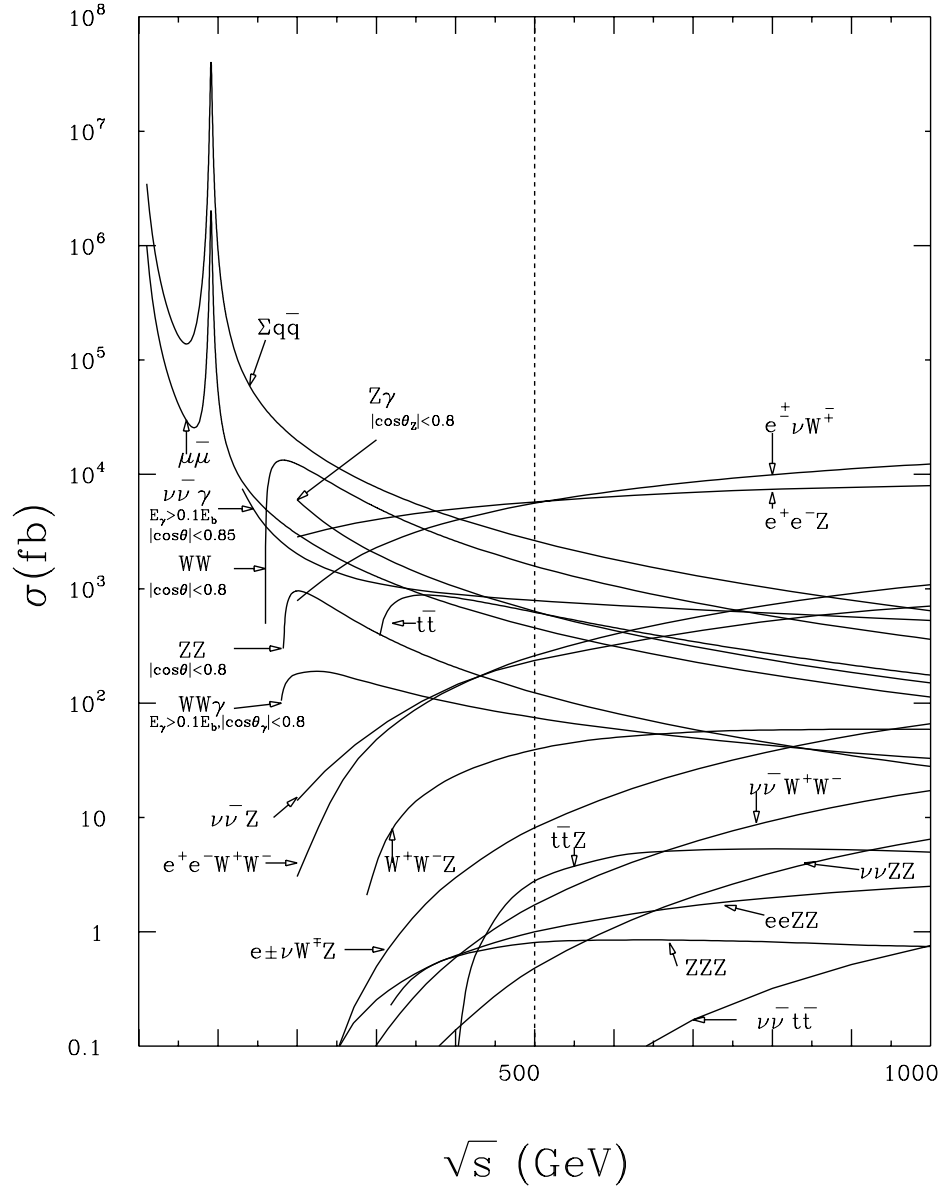
Figure 1: Cross sections for a variety of physics processes at an e^+e^- linear collider, from [60].
