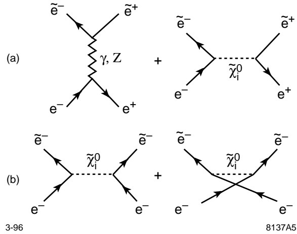
Figure 9: Diagrams contributing to selectron pair production: (a) e^+e^- \rightarrow \tilde{e}^+\tilde{e}^- , (b) e^-e^- \rightarrow \tilde{e}^-\tilde{e}^- .
