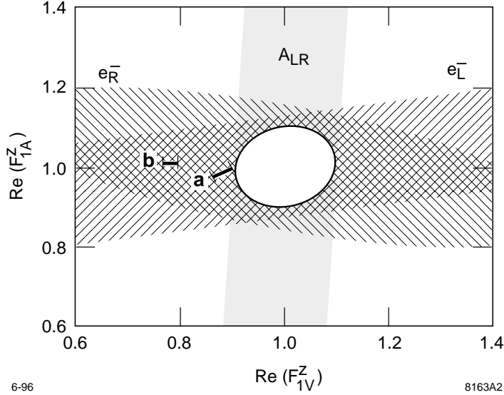
Figure 16: Determination of the form factors for the vector and axial vector couplings of the top quark to the Z , with 100 \text{ fb}^{-1} at 400 GeV [97], compared to the predictions of technicolor models, from [1].
