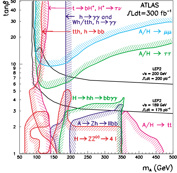
Figure 2: Capability of the ATLAS experiment to study the Higgs sector of the MSSM [62].
