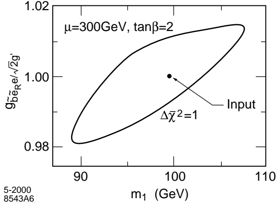
Figure 11: Determination of the g_{b\tilde{e}_R e} coupling from a 100 \text{ fb}^{-1} measurement of selectron pair production, from [80].
