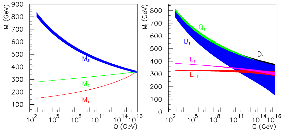
Figure 17: Extrapolation of supersymmetry mass parameters determined at a linear collider from the TeV scale to the grand unification scale, from [117]. The width of each band at the weak scale is the error in the direct parameter determination; these errors are propagated to higher energies using the renormalization group equations.
