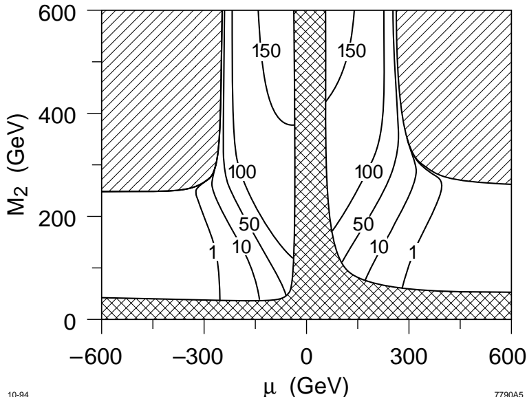
Figure 14: Total cross section for e_R^- e^+ \rightarrow \tilde{\chi}_1^+ \tilde{\chi}_1^- , in fb, as a function of the chargino mass parameters m_2 and \mu .
