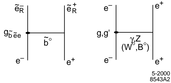
Figure 10: Comparison of the weak interaction coupling g' and its supersymmetric counterpart g_{\tilde{b}\tilde{e}e} .
