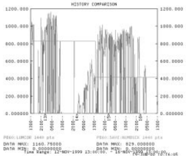
Fig. 1: Luminosity in November of 1999. The luminosity in unit of 10^{30} \text{ cm}^{-2} \text{ s}^{-1} and the number of bunches is plotted versus time. A change in the number of bunches from 829 to 415 decreased the luminosity only slightly from 1100 to 1000 \cdot 10^{30} \text{ cm}^{-2} \text{ s}^{-1} .
