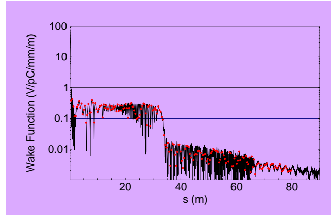
Figure 2: Envelope of Wakefunction with Q \sim Q_{\text{copper}}
