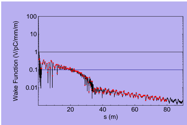
Figure 6: Envelope of Wake Function for Q \sim 200
