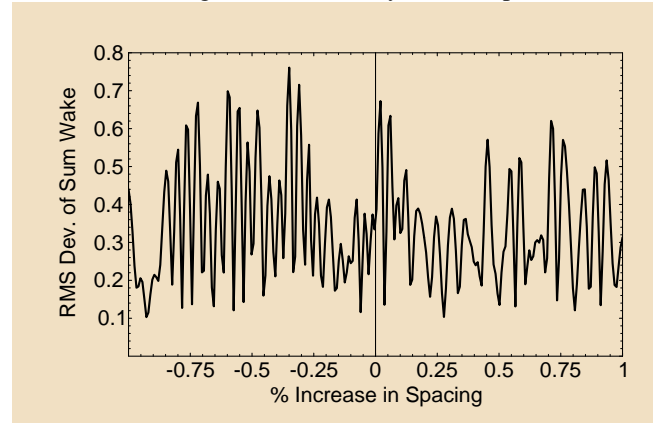
Figure 3: Sum Wake with Q \sim Q_{\text{copper}}
