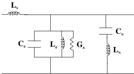
Figure 1: Transmission Line Model of Manifold
