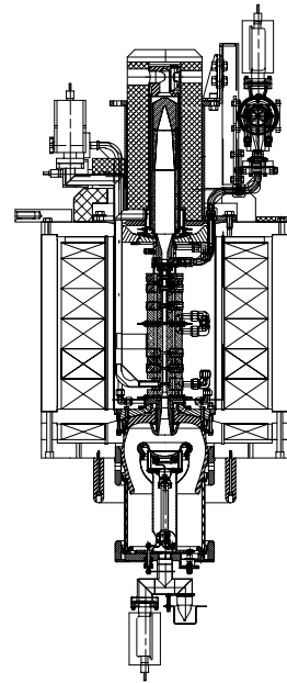
Figure 1: XL-4 Solenoid focused klystron
