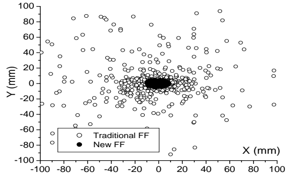
Figure 7: Beam at the entrance of the final doublet for the traditional NLC FF and for the new FF, as determined by particle tracking. Particles of the incoming beam are placed on a surface of an ellipsoid with dimensions N_\sigma(x, x', y, y', E) = (800, 8, 4000, 40, 20) times larger than the nominal beam sizes.
