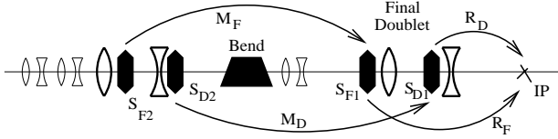
Figure 2: Optical layout of the new final focus.
