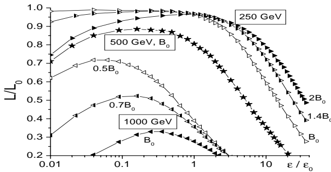
Figure 9: Luminosity versus emittance for different field in the bends and beam energy for the new Final Focus. Tracking includes synchrotron radiation in bends and quadrupoles.
