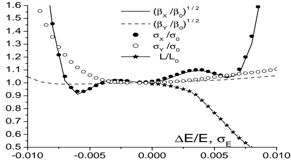
Figure 4: IP bandwidth of the traditional NLC Final Focus. Normalized betatron functions and normalized luminosity equivalent beam size (determined by tracking) versus energy offset \Delta E/E , and normalized luminosity versus rms energy spread \sigma_E .
