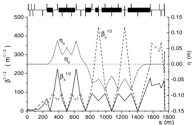
Figure 1: Optics of the traditional Final Focus for the Next Linear Collider showing horizontal and vertical betatron ( \beta ) and dispersion ( \eta ) functions. Focusing and defocusing quadrupoles are indicated as up and down bars on the magnet plot above the optics, while the bends are centered.
