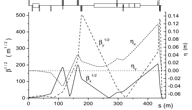
Figure 3: Optics of the new NLC Final Focus System showing horizontal and vertical betatron ( \beta ) and dispersion ( \eta ) functions similarly to Fig.1.
