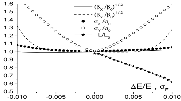
Figure 5: IP bandwidth of the New NLC Final Focus with definitions as in Fig.4.
