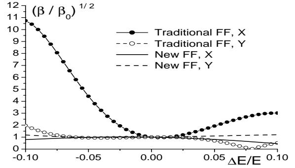
Figure 6: FD bandwidth of the Traditional and New NLC Final Focus. Normalized betatron functions at the final doublet versus energy offset \Delta E/E .
