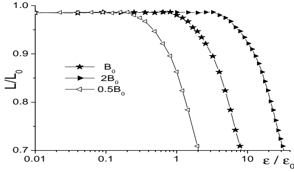
Figure 8: Luminosity versus emittance for the new Final Focus for the nominal, twice larger and twice lower field in the bends. Tracking without synchrotron radiation.
