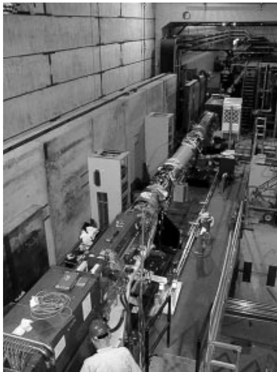
Figure 2: The PEP-II interaction region, before roll-in of the BaBar detector.
