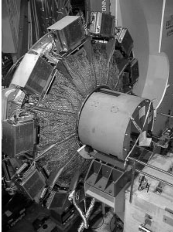
Figure 5: Phototube array for the BaBar DIRC particle identification system.
