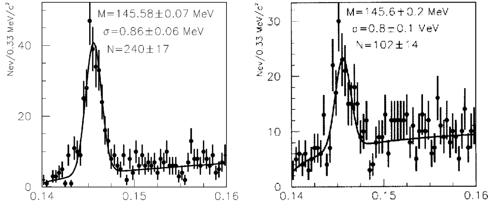
Figure 13: D^*-D^0 mass difference, as reconstructed by the BaBar detector. Left: D^0 \rightarrow K^\pm \pi^\mp ; Right: D^0 \rightarrow K^\pm \pi^\mp \pi^0 .
