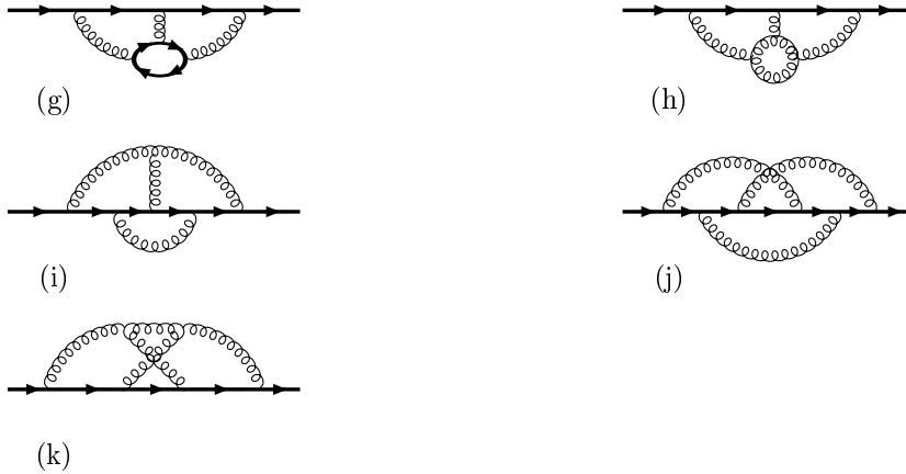
FIG. 1. Examples of three-loop quark propagator diagrams corresponding to eleven integration topologies.
