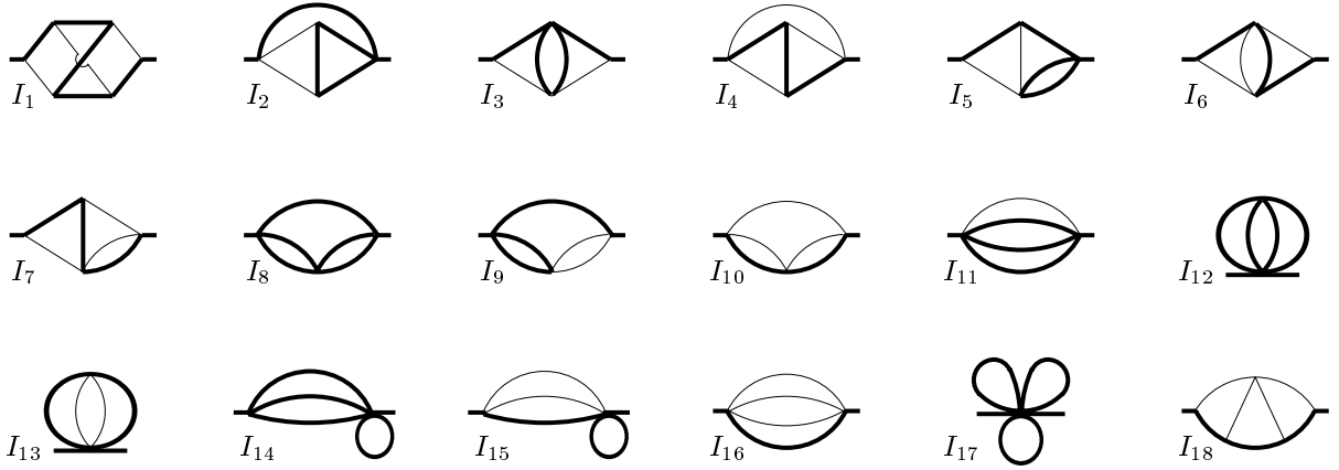
FIG. 2. Pictorial representation of the complete set of primitive 3-loop on-shell integrals I_1 - I_{18} . Thick lines are used to indicate massive scalar propagators and thin lines indicate massless propagators.
