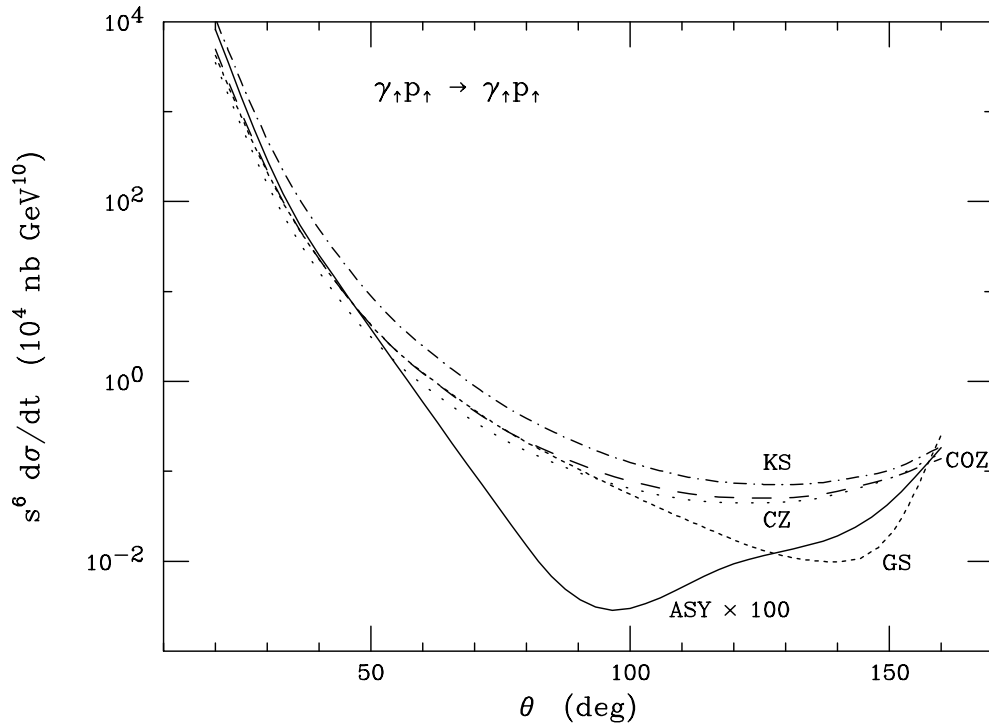
Figure 2: The cross section for \gamma_{\uparrow}p_{\uparrow} \rightarrow \gamma_{\uparrow}p_{\uparrow} for five different distribution amplitudes, CZ, COZ, KS, GS and ASY. The results for the asymptotic distribution amplitude (ASY) have been multiplied by 100.
