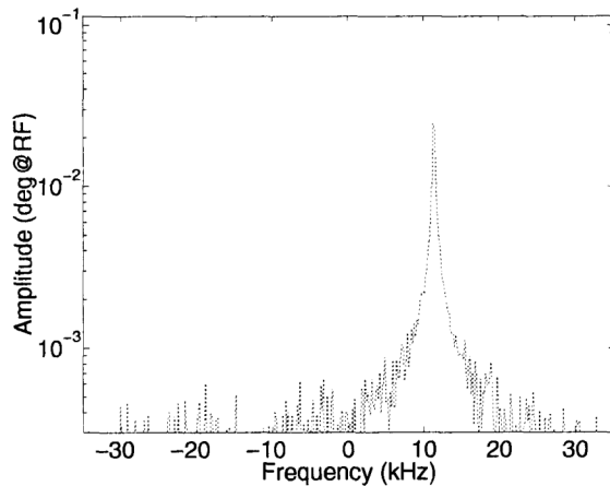
Figure 3: 70 kHz section of the high resolution spectrum in Fig. 2, showing an unstable upper sideband and a damped lower sideband at 204f_{rev} .
