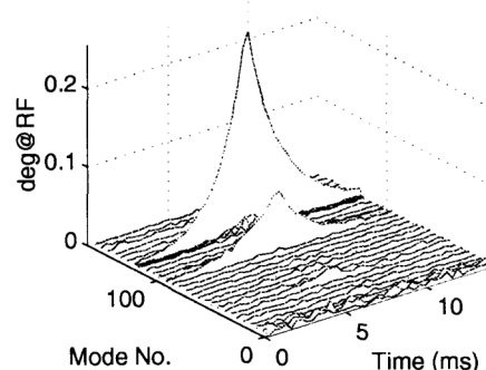
Figure 1: Plot of a turn by turn FFT of the bunch data, revealing two unstable modes (mode 95 and 124) of 328 bunches in the ALS over a 12 ms time interval. The feedback system is on for t < 0 and t > 6 ms, and off for 0 < t < 6 ms. Unstable bunch motion grows during the feedback off interval. The total machine current was 120 mA.
