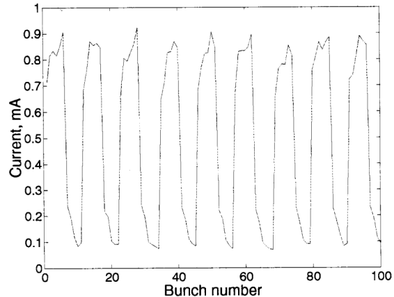
Figure 5: Current measurement for a square wave fill
