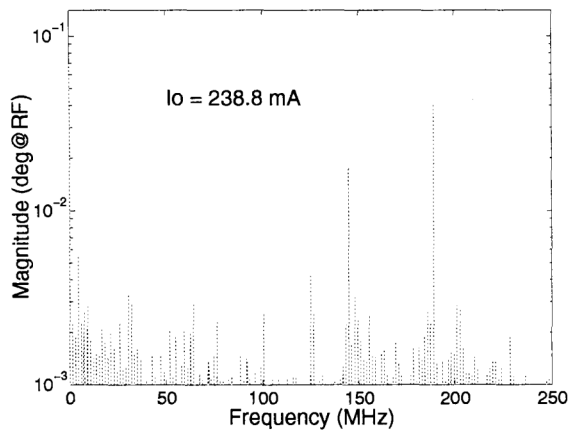
Figure 2: Magnitude of high-resolution FFT of growing transient in Fig. 1, showing all the spectral components over a 250-MHz bandwidth.
