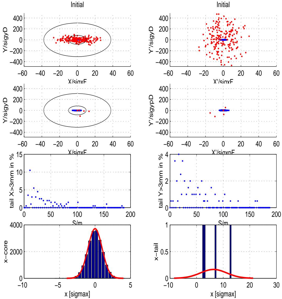
FIGURE 23. This Figure for the pre-linac is different from the ones shown before, in as much as it shows the initial distribution in x - y and x' - y' space, (subfigure a and b), the same parameters after collimation (subfigures c and d), the loss process along the accelerator in both x and y (subfigures e and f), and the x -core and x -tail after collimation (subfigures g and h). The core (20000) and Halo particles (200) were created with the total tail method explained above. The circles in subfigures a and c are the beam stay clear (inner circle, here a 10 \sigma radius) and the collimation radius used (3 mm radius, outer circle). As explained earlier in the text the main reason for doing the simulation with a total tail approach, rather than the Halo Ring approach, is to test graphically if there is bleeding from the core into the tails. None did. One also has to test if particles get beyond the BSC without being removed beyond 3 mm. 2 out of 200 (2%) did. Note again, as described in the text, that the Halo corresponds to an exponential distribution in J -space starting at (the equivalent of) 3.29 \sigma in both x and y , and that the width of the Halo distribution is 10 times the width of the core.
