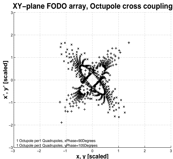
FIGURE 9. Phase space plot of one particle in x and y phase space. The particle goes through a 100 cell FODO lattice with a phase advance of 90 and 105^\circ in x ( x 's) and y ( + 's), respectively. This simulation was performed with a full coupled matrix multiplication. The figure has to be interpreted as the (one) particle initially being on its unperturbed phase ellipse(s), then slowly spiraling out under the relentless kicks of the Octupoles, until it is abruptly lost.
