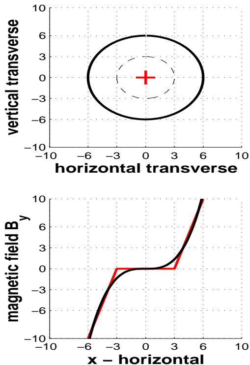
FIGURE 1. The top part shows the conceptual division of an accelerator in two concentric parts, with their separate lattices. Since this is physically not possible, ideally magnetic elements have to be found which are zero in the center and linear in the Halo region (light curve in the lower part). Maxwell's equations make this also impossible, so a compromise, here an Octupole field, is shown (dark curve in the lower part). But theoretically, see below, higher order multipoles have to be even better, although physically more difficult to build. It should strongly be emphasized that non-linear RF fields also should be considered.
