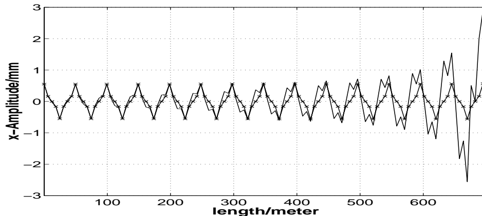
FIGURE 4. Although only one coordinate is shown here, this calculation was done for a realistic Octupole field with the required cross coupling terms in x and y. The single particle motion in the linear (Quadrupoles only) and non-linear (Quadrupoles and Octupoles) case are compared. The starting value was x = 600\mu\text{m} (corresponding to 9\sigma in the NLC main linac) and x' = 0 . The positions of the Quadrupoles is indicated with x's in the linear case. This curve shows the very regular even pattern of a constant 90^\circ FODO lattice. The added kicks of the Octupoles have the effect of changing the effective phase advance to higher values. The amplitude changes, slowly at first, then rapidly, until the particle gets lost at about 3 mm of amplitude. Note that this combined phase advance depends strongly on the position in x,y space, making predictions of when a particle will get lost close to impossible in general. This example was calculated with the standard NLC main linac lattice cell length of 12.5 m and Octupoles with a 3kG pole tip field at a pole tip radius of 5 mm ( k_3 = 43300\text{m}^{-3} in MAD notation).
