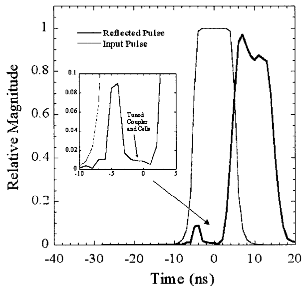
Figure 6: Coupler VSWR in the time domain.
