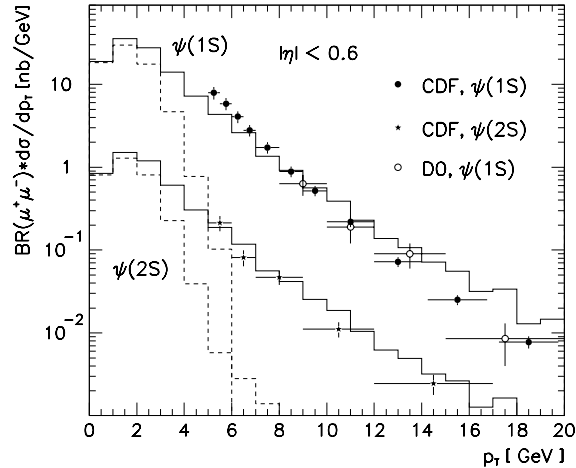
Figure 3. Transverse momentum spectra of prompt charmonium ( J/\psi and \psi' ) in p\bar{p} collisions at the Tevatron energy. Data from CDF and D0 compared to results from the SCI model (histograms) applied to c\bar{c} production from leading order ( \alpha_s^2 ) matrix elements (dashed lines) and with inclusion of higher order contributions calculated in the parton shower approach (full lines). From [12].
