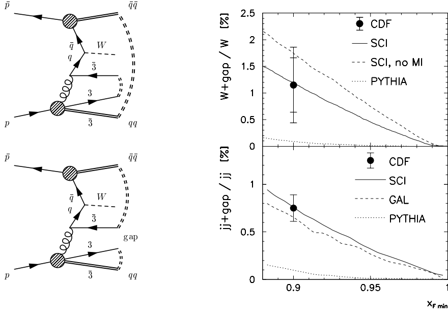
Figure 2. W production in p\bar{p} with string topology before and after colour rearrangement resulting in a gap. Relative rate of W and two-jet ( jj ) events with a rapidity gap corresponding to diffraction with a leading proton with minimum x_F = 0.9 in Tevatron data [11] and in the SCI and GAL models. Sensitivity to multiparton interactions (MI) and results from standard PYTHIA without soft colour exchanges is also shown [10].
