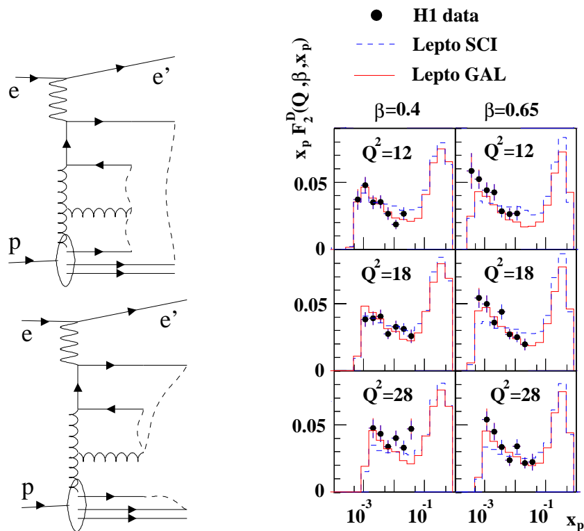
Figure 1. Gluon-induced deep inelastic scattering event with examples of colour string connection (dashed lines) of partons in conventional Lund model [5] based on the colour order in pQCD (upper left), and after colour rearrangement through SCI or GAL mechanisms (lower left). The diffractive structure function F_2^{D(3)}(x_P; \beta, Q^2) in a selected kinematic range with H1 data [8] compared to the SCI and GAL models; excerpt from [7].
