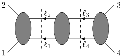
Figure 3: The s -channel double two-particle cut of a two-loop amplitude separates it into a product of three tree amplitudes. The dashed lines represent the generalized cuts.
