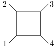
Figure 11: C_{1234}^{1\text{-loop}} is given by dressing each vertex in the figure with \tilde{f}^{abc} , and dressing each bond between vertices with a \delta^{ab} .
