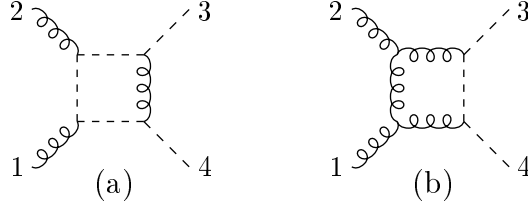
Figure 8: Representative planar diagrams for the subleading-in-color (a) and leading-in-color (b) one-loop amplitudes for two gluons and two scalars. The diagrams are divided into the two classes according to whether or not there is an internal gluon line to the right of the scalar line.
