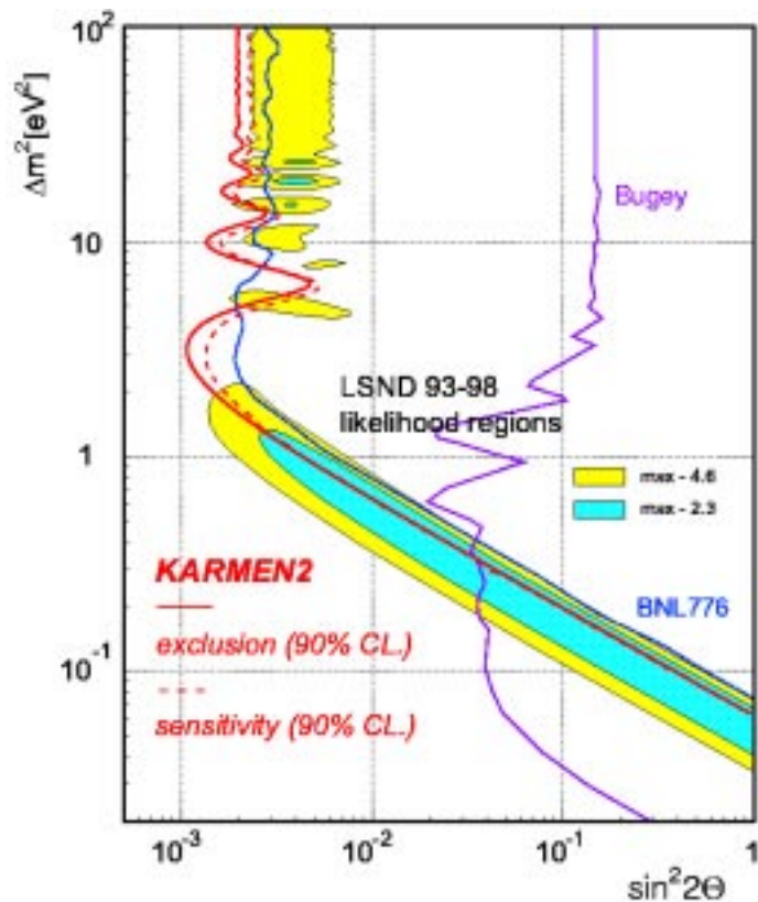
Figure 2: Electron neutrino experimental results. LSND is not in conflict with other experiments in a band from \Delta m^2 of 0.3 eV^2 and \sin^2 2\theta of 3 \times 10^{-2} to \Delta m^2 of 1 eV^2 and \sin^2 2\theta of 1.5 \times 10^{-3} . [4]
