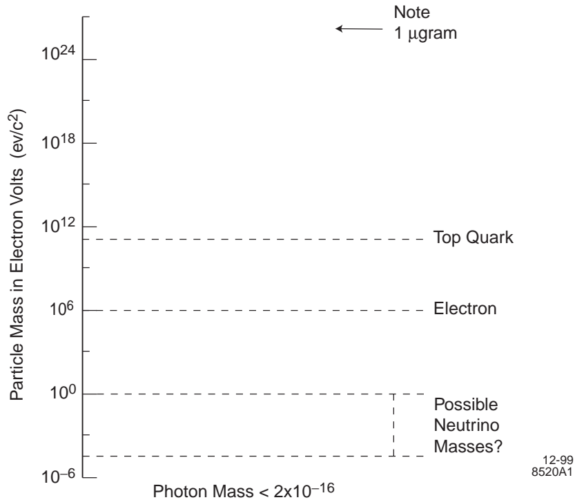
Figure 2: The range of the masses of the known elementary particles.
