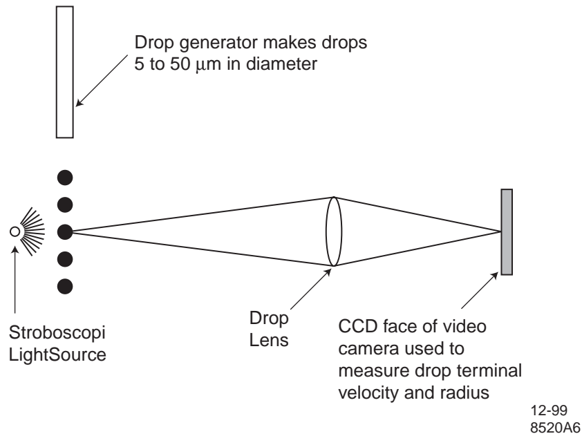
Figure 6: Schematic illustration of liquid drop apparatus for searching for massive particles.
