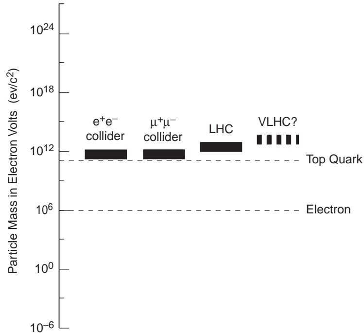
Figure 3: Upper limits of direct mass searches for accelerators being constructed or proposed.
