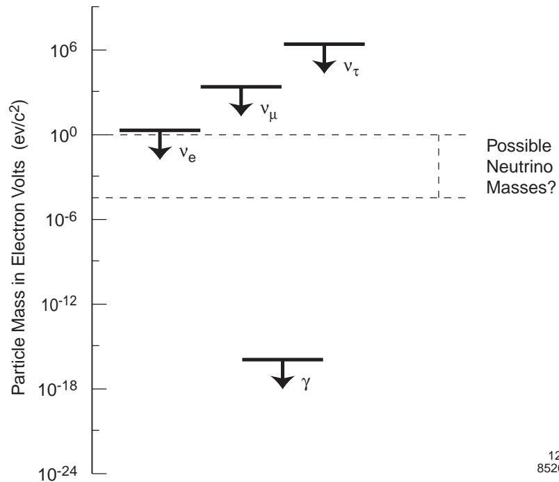
Figure 8: Our scanty knowledge of the masses of the known, light, neutral particles.
