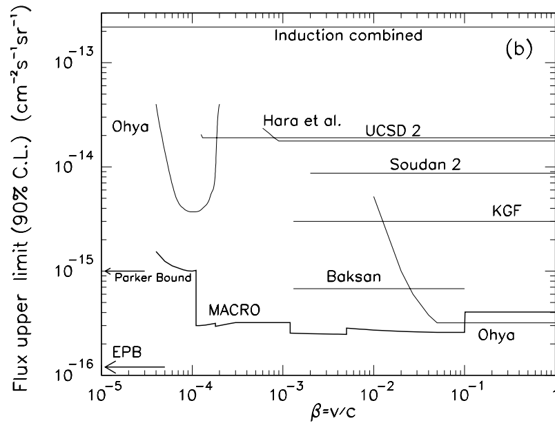
Figure 10: Measured upper limits on monopole fluxes compiled [9].
