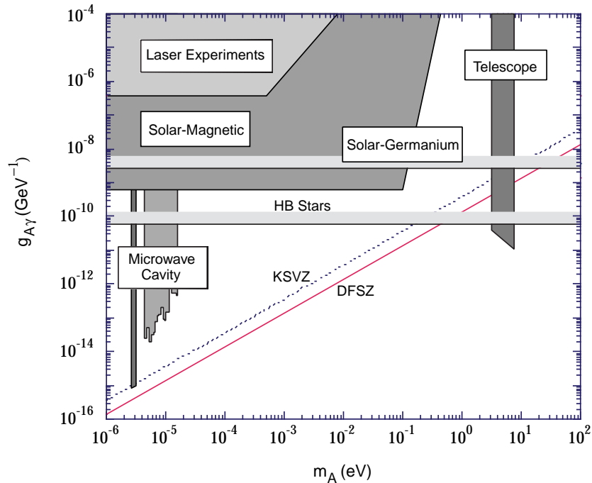
Figure 9: Unexplored axion search regions in g_{A\gamma}-m_A space where g_{A\gamma} is the axion coupling constant and m_A is the axion mass [7].
