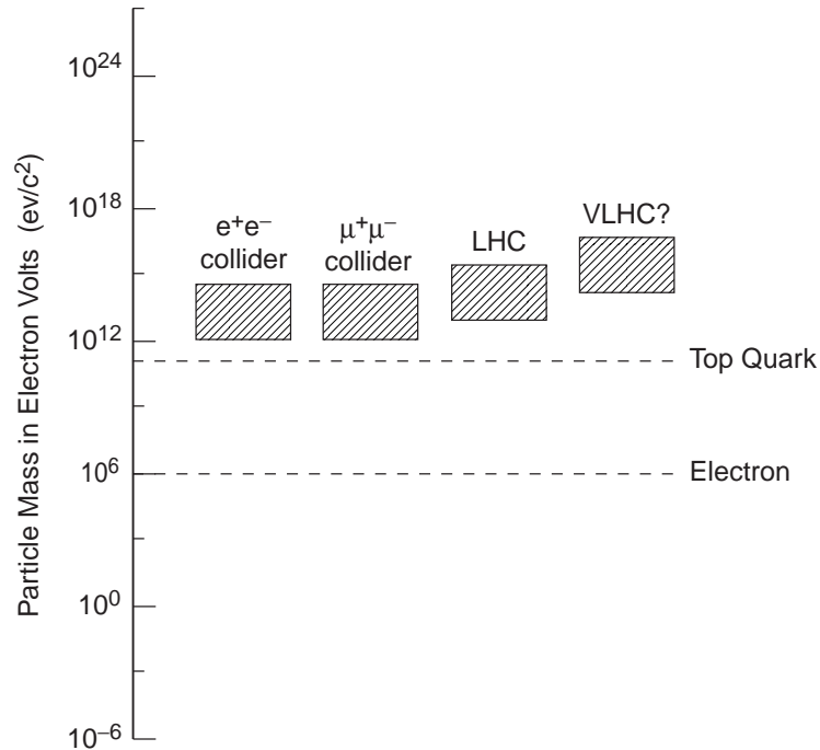
Figure 4: Upper limits of indirect mass searches for accelerators being constructed or proposed.
