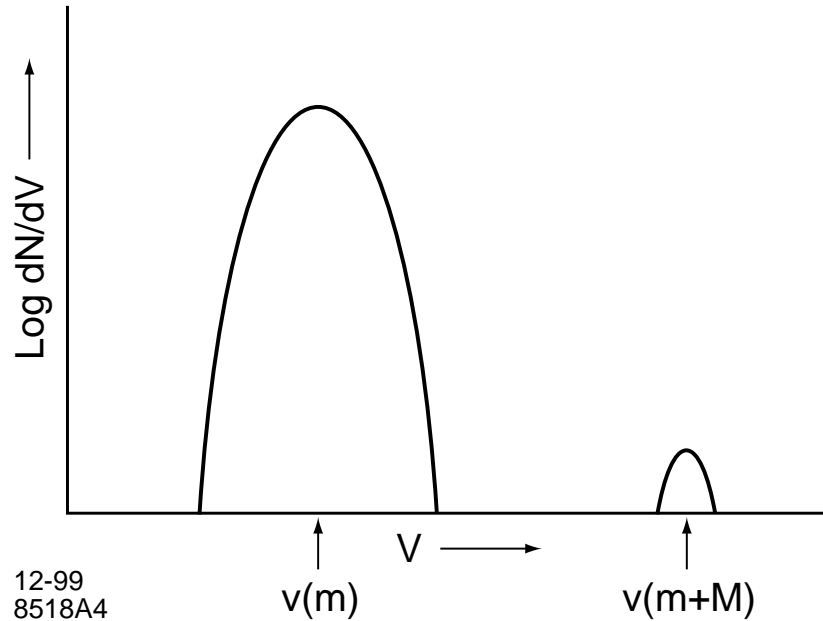
Figure 7: Illustrative plot of number of drops dN/dv versus v , with a very large peak at v(m) and a relatively very small peak at v(m + M) .
