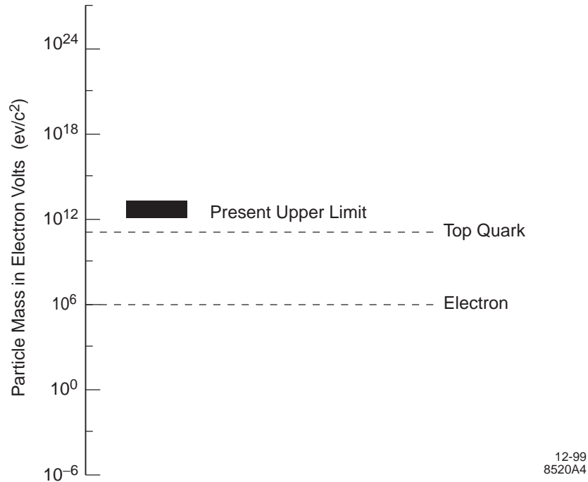
Figure 5: Upper limit of searches for massive particles using mass spectrometry to look for unusually heavy atoms.
