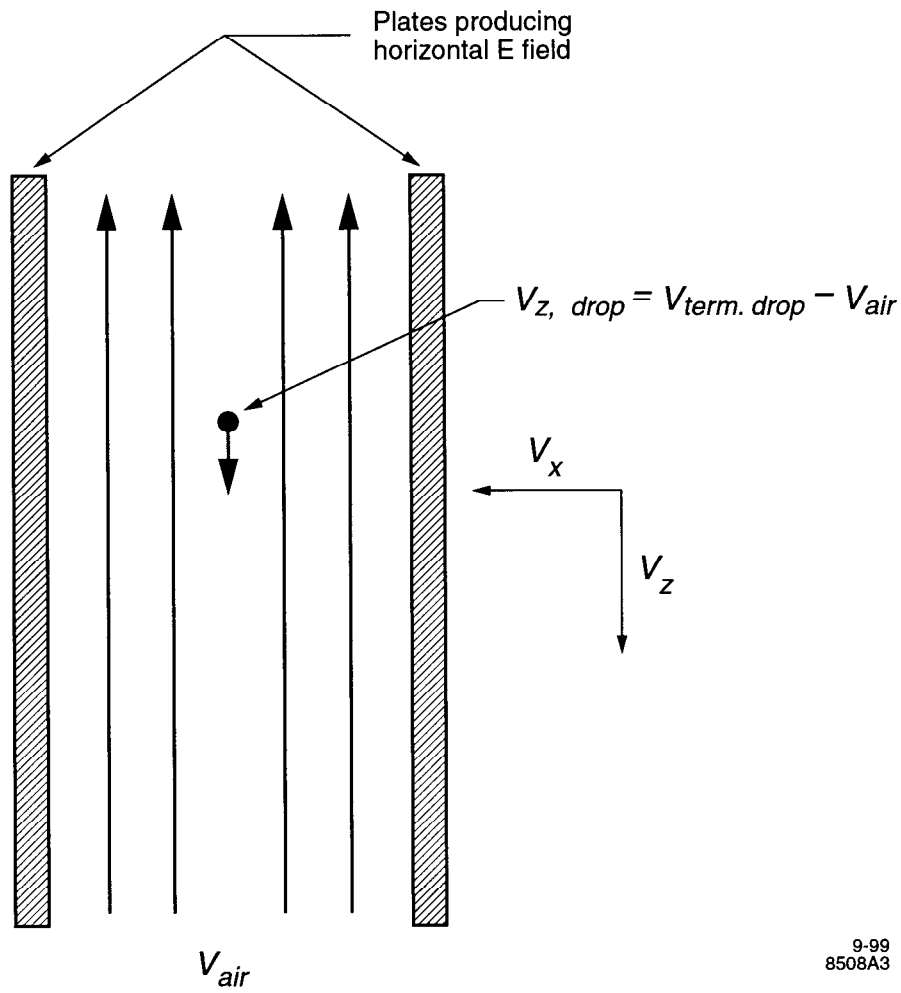
Fig. 3. Schematic illustration of the use of upward airflow to reduce drastically the downward vertical velocity, v_{z,drop} , of the drop. The view is along the axis of the optical system.
