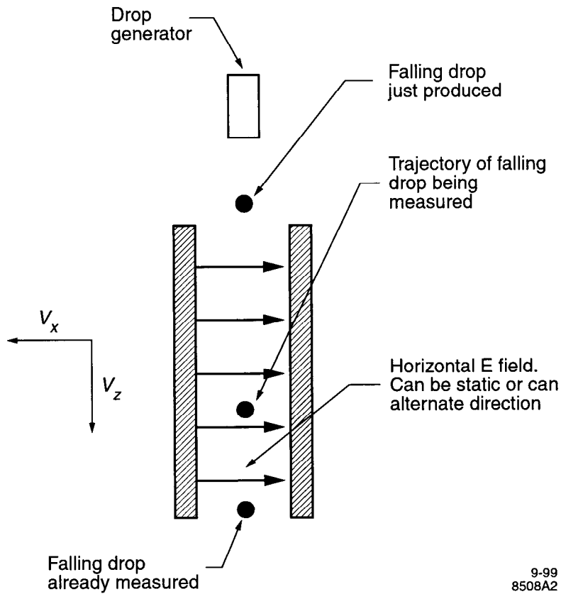
Fig. 2. Schematic illustration of the use of a horizontal electric field. The view is along the axis of the optical system.
