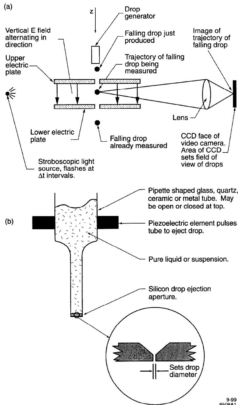
Fig. 1. (a) Schematic vertical view of our traditional Millikan method apparatus. (b) Explanatory view of the piezoelectric drop generator. The diameter of the hole in the drop ejection aperture plate sets the diameter of the drop within a range of about \pm 15\% . The exact diameter depends upon aperture shape, pulse shape, and pulse frequency
