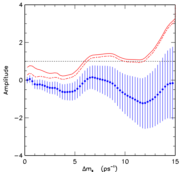
Figure 8: Amplitude distribution for CDF's \phi/l analysis.
