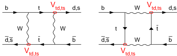
Figure 1: B\bar{B} mixing diagrams.
