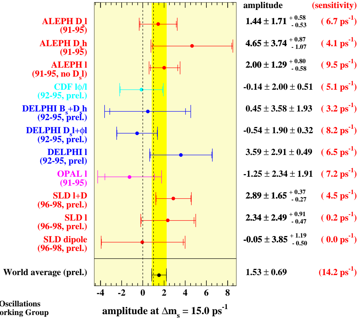
Figure 11: Measured amplitude at \Delta m_s = 15 \text{ ps}^{-1} for each analysis.
