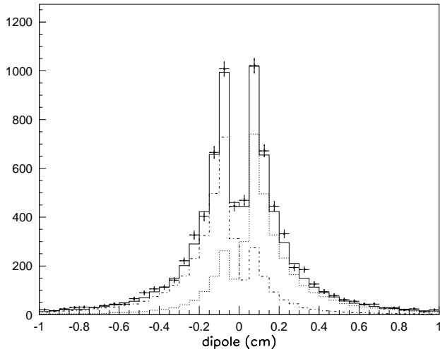
Figure 13: SLD's dipole charge distribution for data (points) and Monte Carlo (histogram). The dotted and dashed histograms represent the b - and \bar{b} components, respectively.
