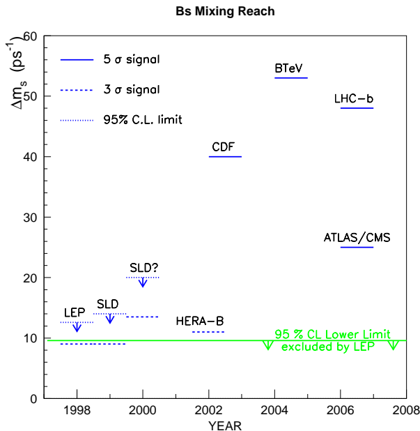
Figure 15: Expected B_s mixing reach for future-generation B physics experiments.
