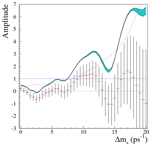
Figure 7: Amplitude distribution for DELPHI's D_s l analysis.
