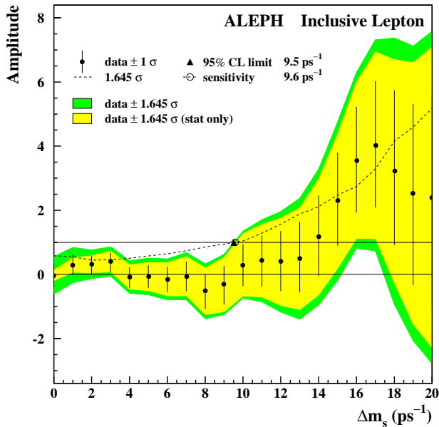
Figure 5: Amplitude distribution for ALEPH's inclusive lepton analysis.
