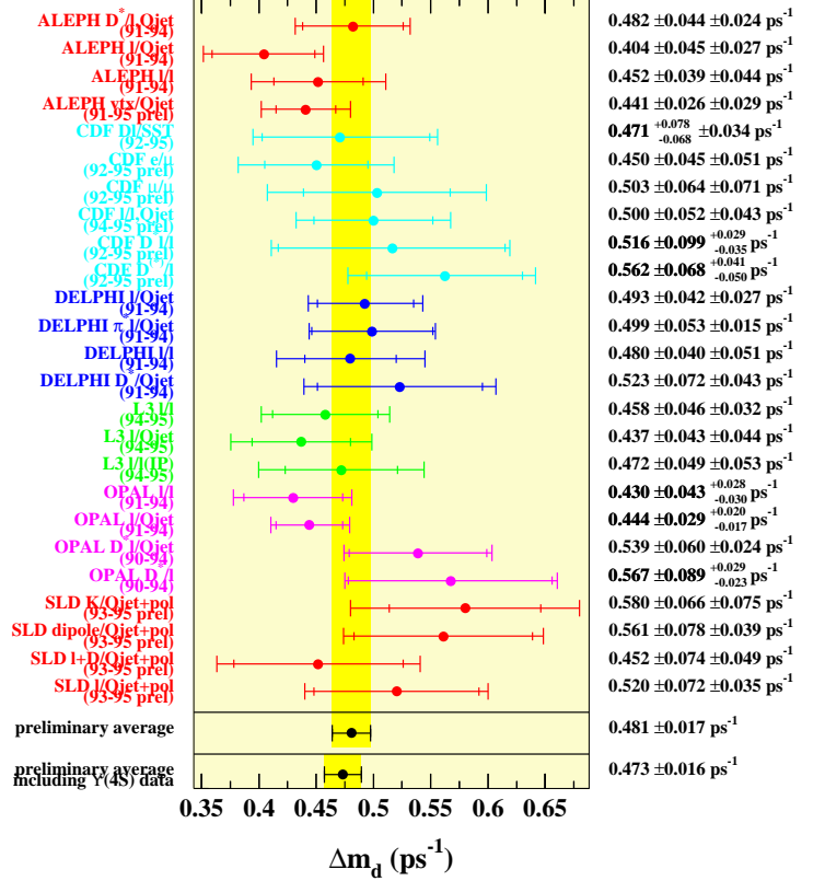
Figure 4: Measurements of \Delta m_d .
