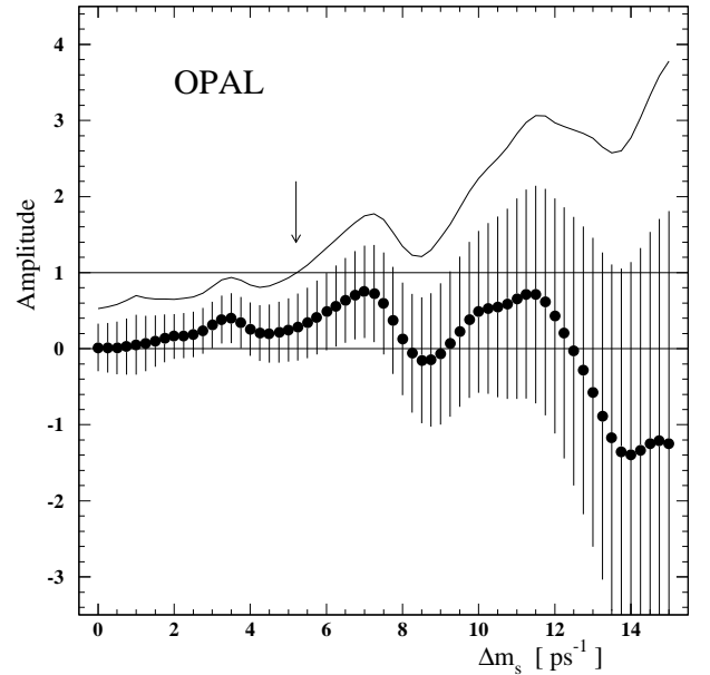
Figure 6: Amplitude distribution for OPAL's inclusive lepton analysis.
