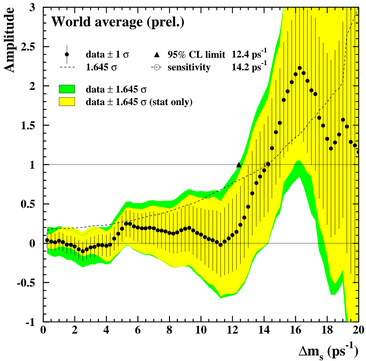
Figure 12: World average amplitude vs. \Delta m_s distribution.
