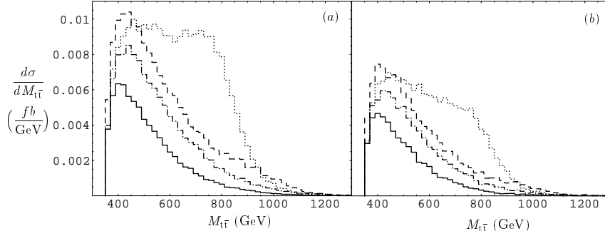
Figure 1: (a) Differential cross section for e^+e^- \rightarrow \nu t\bar{t} as a function of the t\bar{t} invariant mass, for a LC with \sqrt{s} = 1.5 TeV. The curves correspond to the SM with a Higgs mass of 100 GeV (solid) and 800 GeV (dots), the technicolor model described in the text with m_\rho = 1 TeV (dash) and the LET limit (dot-dash). (b) Same as (a) including ISR and beamstrahlung.
