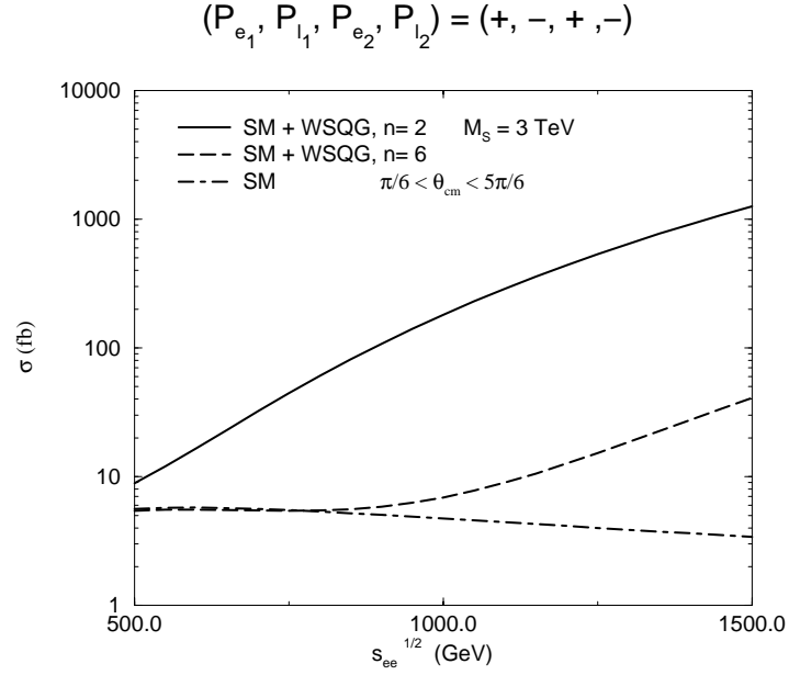
Figure 3: SM + WSQG and SM cross sections for the (+, -, +, -) polarization. Here, M_S = 3 \text{ TeV} and n = 2, 6 , for the WSQG contributions.
