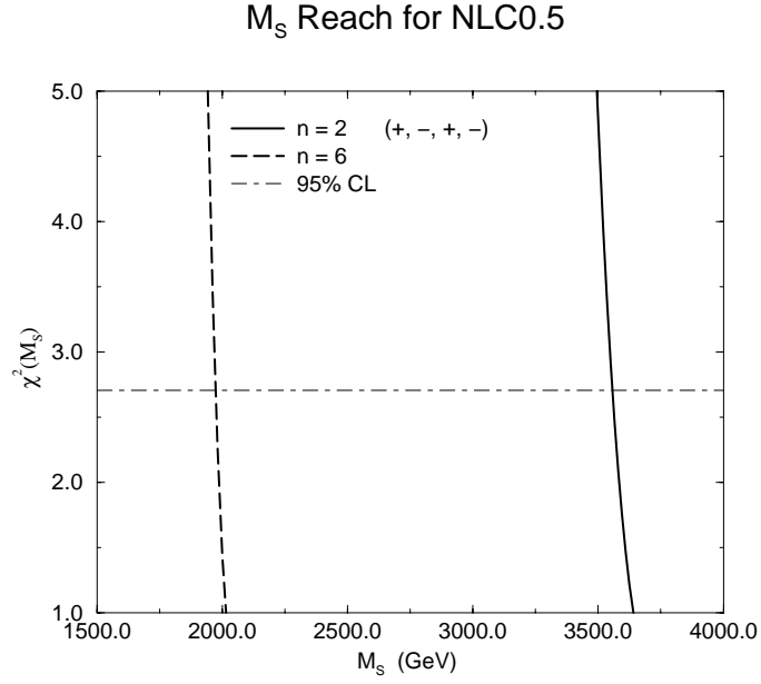
Figure 5: The M_S reach for NLC0.5. The solid and the dashed lines represent the \chi^2 as a function of M_S for the cases n = 2 and n = 6 , respectively. The dot-dashed line marks the reach at the 95% confidence level.
