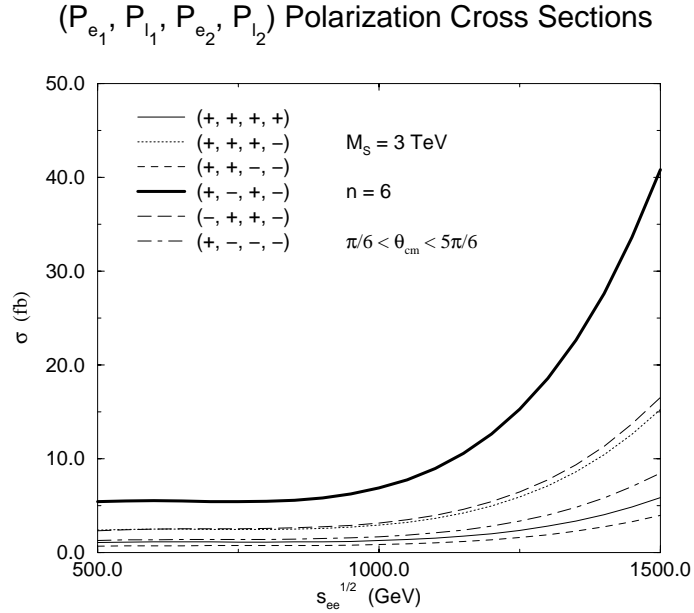
Figure 1: SM+WSQG and SM cross sections, represented by the thick and the thin lines, respectively, for the initial helicities ++ and +- . The gravity contribution is calculated for M_S = 3 TeV and n = 6 .
