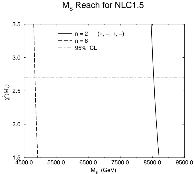
Figure 7: The M_S reach for NLC1.5. The solid and the dashed lines represent the \chi^2 as a function of M_S for the cases n = 2 and n = 6 , respectively. The dot-dashed line marks the reach at the 95% confidence level.
