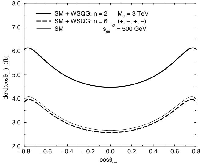
Figure 4: SM + WSQG and SM differential cross sections at \sqrt{s_{ee}} = 500 \text{ GeV} for the (+, -, +, -) polarization. Here, M_S = 3 \text{ TeV} and n = 2, 6 , for the WSQG contributions.
