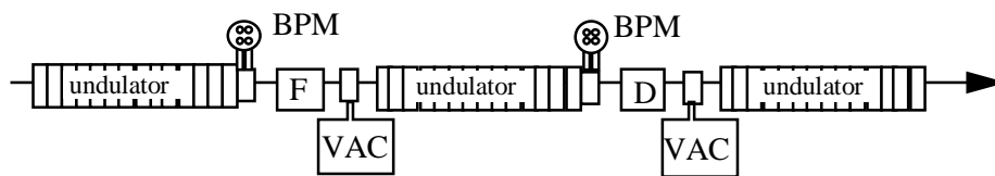
Fig. 7 . Schematic view of undulator structure.
