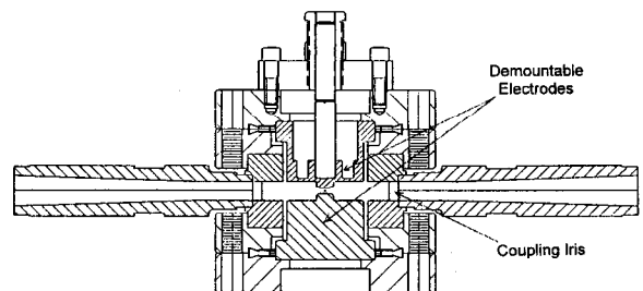
Fig. 4. TM 020 RF breakdown test cavity assembly
