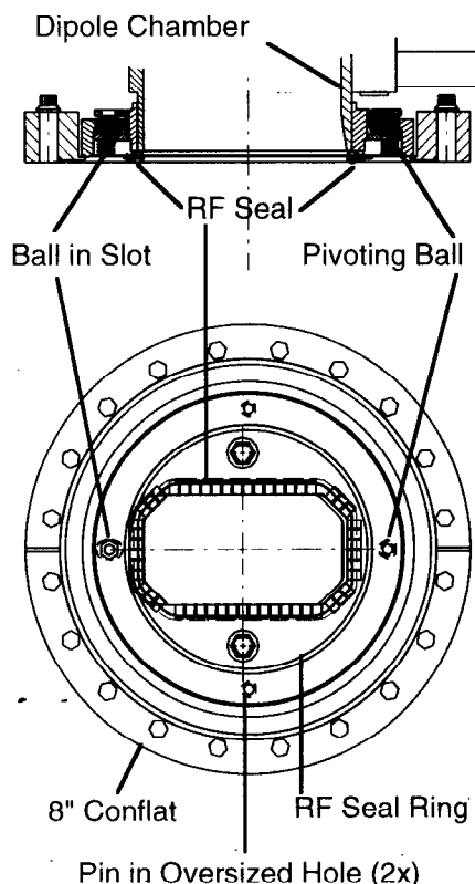
Figure 2. Flex Flange Assembly with Integral RF Seal
