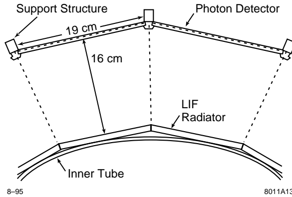
Fig. 13. A schematic end view of two sectors of the CLEO III Fast RICH detector. Not shown is the situation at polar angles near 90^\circ , where the LiF radiators must be tilted by 20^\circ to allow the Cherenkov cone to emerge with reasonable efficiency.
