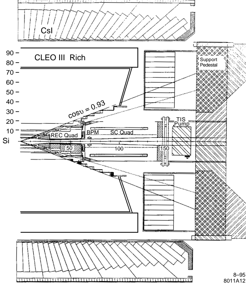
Fig. 12. An elevation view of one-half of the CLEO III detector.
