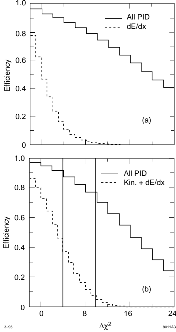
Fig. 3. The efficiency for accepting an event as a function of the \chi^2 difference between events containing a (\pi^+\pi^-) hypothesis and those containing a kaon; the dashed line shows the simulated performance without the PID system, while the solid line adds the DIRC and forward ATC systems of BABAR : (a) B^0 \rightarrow \pi^+\pi^- . (b) B^0 \rightarrow \rho^+\pi^- .
