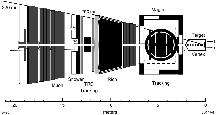
Fig. 15. Plan view of the HERA B detector.
