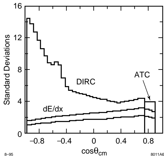
Fig. 6. The predicted K/\pi separation performance for the BABAR systems, in standard deviations versus the cosine of the center-of-mass polar angle, for pions from the reaction B^0 \rightarrow \pi^+\pi^- . The two curves labeled dE/dx indicate the range expected for separation using different models of the tracking chamber.
