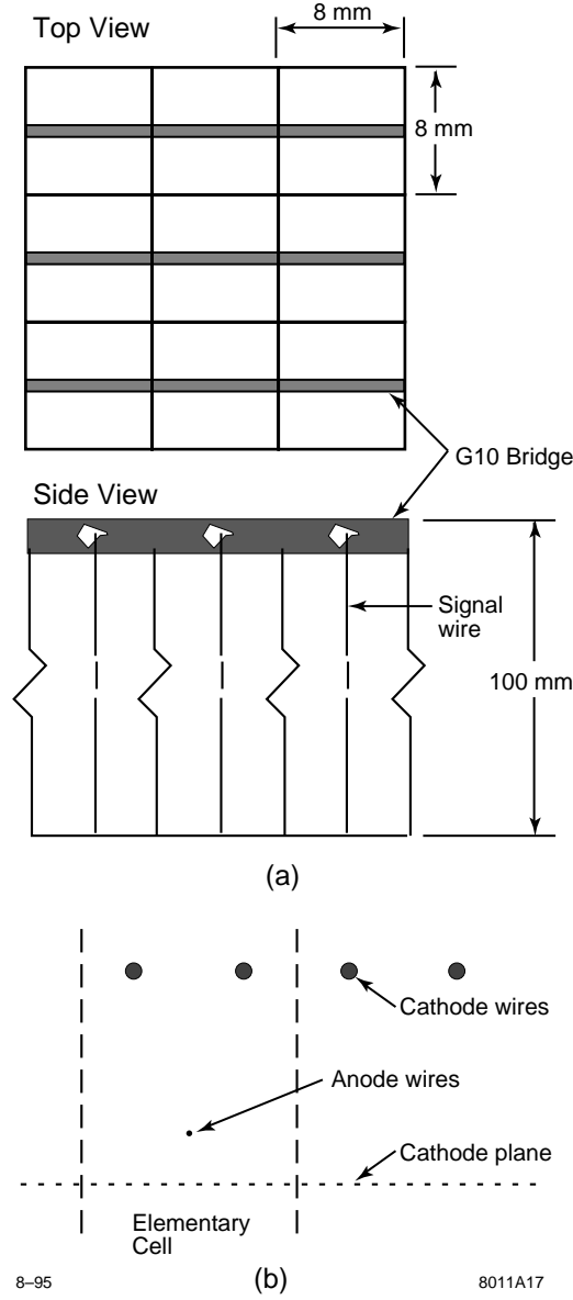
Fig. 17. Schematic views of the geometry of the photodetection chambers for the HERA B RICH: (a) with a TMAE photocathode, (b) with a CsI photocathode.
