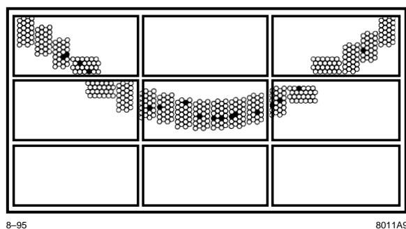
Fig. 9. Online display of a typical event in Prototype-II at a track dip angle of 20^\circ .
