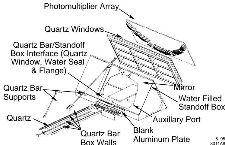
Fig. 8. Isometric view of the Prototype-II detector.
