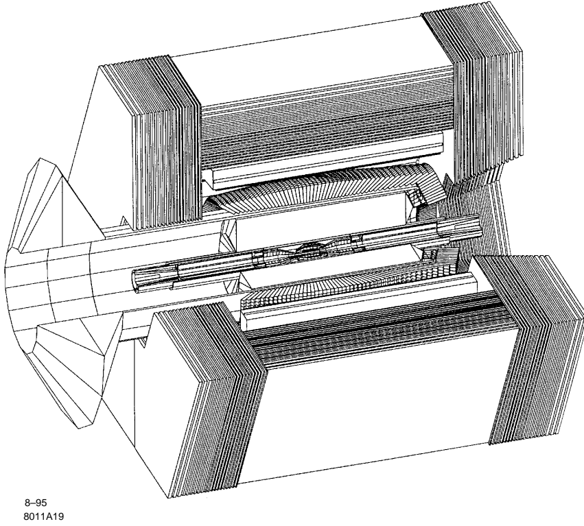
Fig. 4. A three-dimensional view of BABAR .
