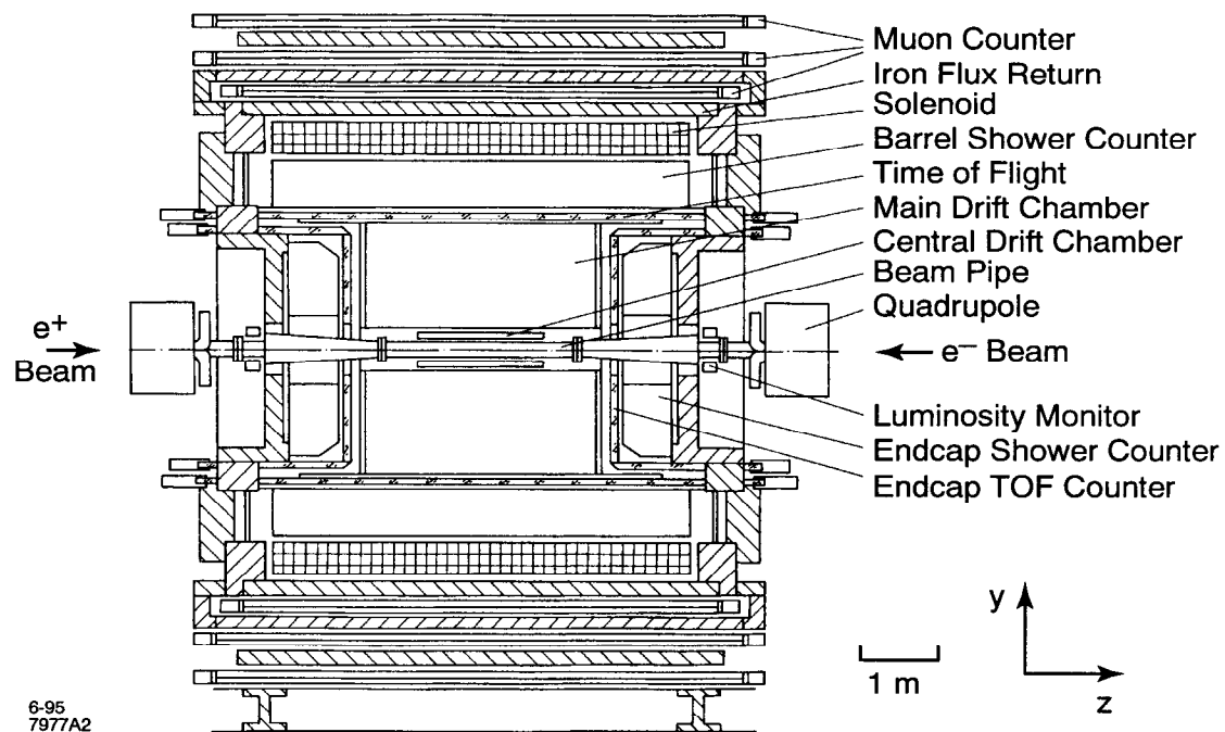
FIG. 2. The Beijing Spectrometer (BES) in y - z projection.
