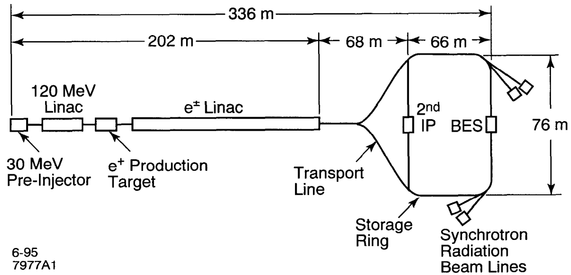
FIG. 1. The Beijing Electron-Positron Collider (BEPC). The 202 meter injection linac leading to the 240 meter circumference storage ring is shown at the left. The electrons circulate clockwise, and the positrons counter-clockwise. The BES sits on the side of the ring opposite the injection linac.
