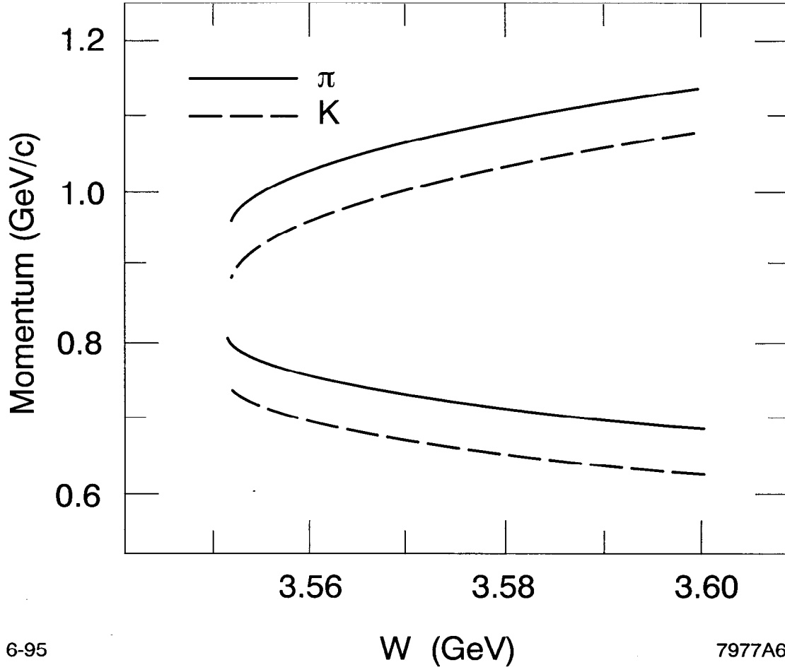
FIG. 6. The momentum limits as a function of c.m. energy, W , for pions and kaons for the decays \tau \rightarrow \pi\nu and \tau \rightarrow K\nu respectively, obtained using a \tau mass value of 1775.9 MeV, as discussed in the text.
