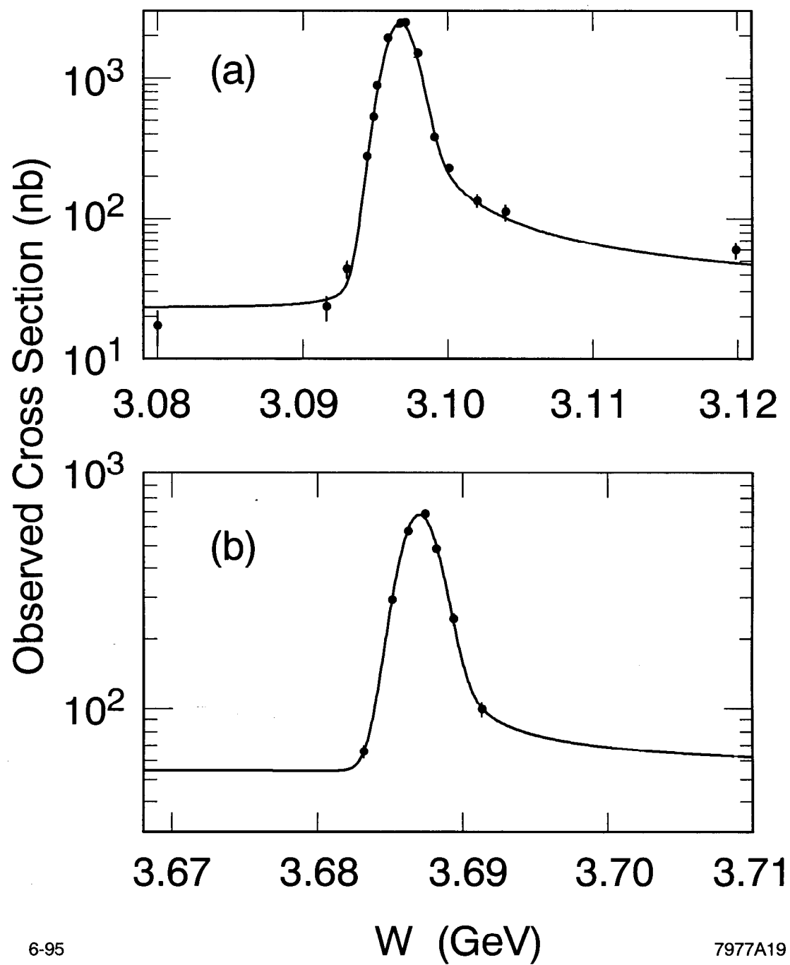
FIG. 19. The results of typical scans, taken during the experiment, of (a) the J/\psi resonance, and (b) the \psi' resonance; W is the c.m. energy.
