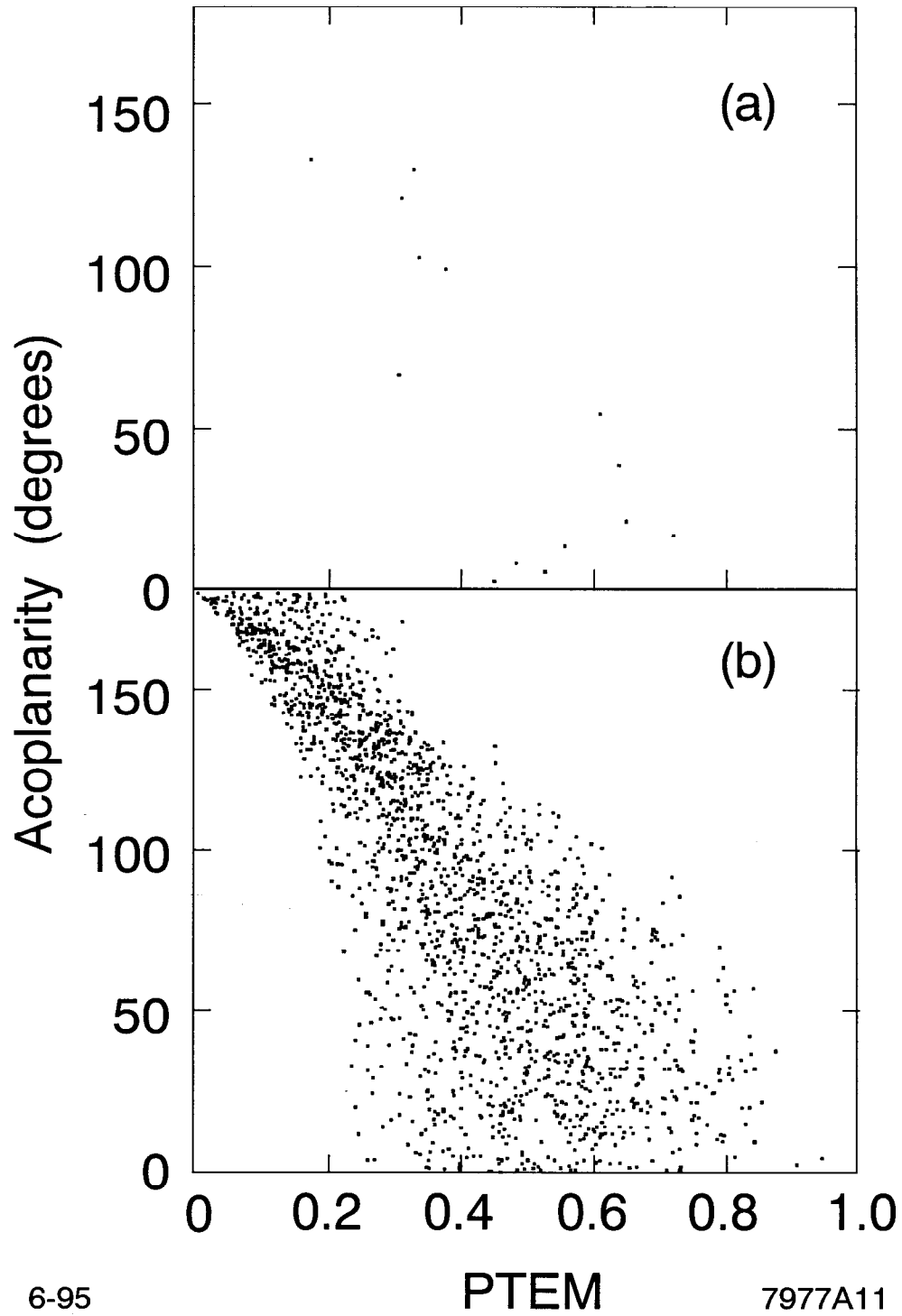
FIG. 11. (a) The scatterplot of PTEM vs. Acoplanarity for the \tau^+\tau^- candidate e\mu events. (b) The same scatterplot for e\mu events obtained from the \tau^+\tau^- Monte Carlo simulation after the application of the same selection criteria.
