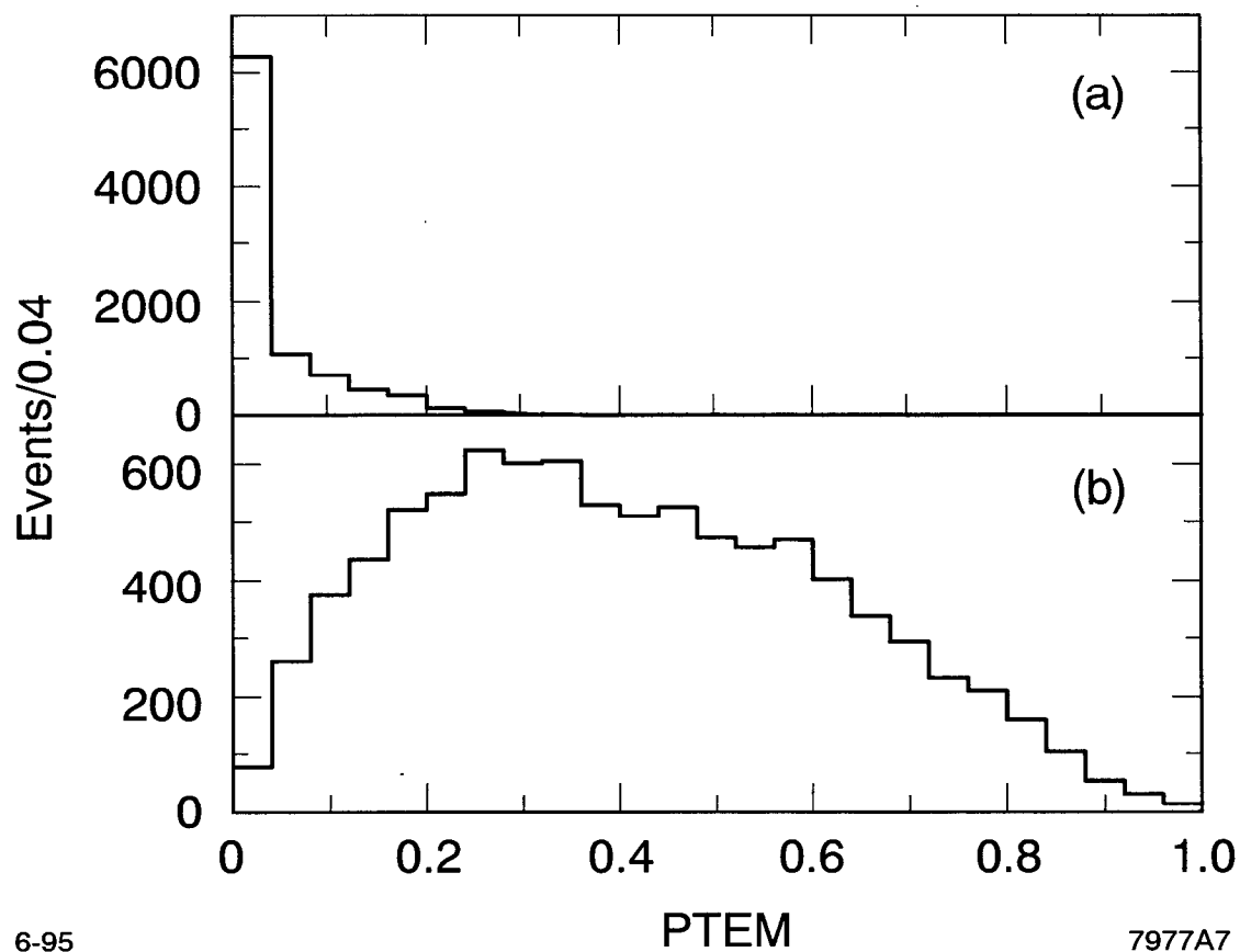
FIG. 7. The distribution in the variable PTEM for (a) the \tau^+\tau^- candidate sample after the application of the particle identification criteria, and (b) \tau^+\tau^- events from the Monte Carlo simulation selected by the same criteria.
