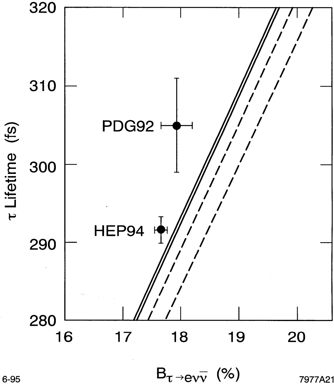
FIG. 21. The variation of the \tau lepton lifetime, t_\tau , with B_{\tau \rightarrow e \nu \bar{\nu}} given by Eq. (6) under the assumption of lepton universality; the \pm 1\sigma bands obtained by using the value of m_\tau from the present analysis (solid lines), and by using the PDG92 value [10] (dashed lines), are shown in comparison to the points ( 1\sigma error bars) corresponding to the current average values of t_\tau and B_{\tau \rightarrow e \nu \bar{\nu}} (HEP94 [17]) and the PDG92 values.
