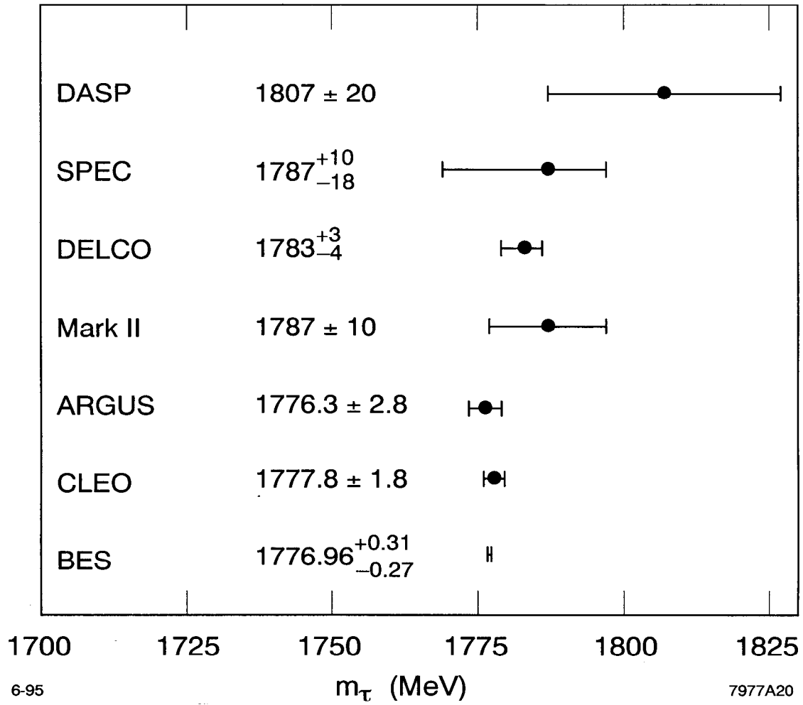
FIG. 20. A comparison of the value of the mass of the \tau lepton obtained from the present analysis to the results from other experiments [2].
