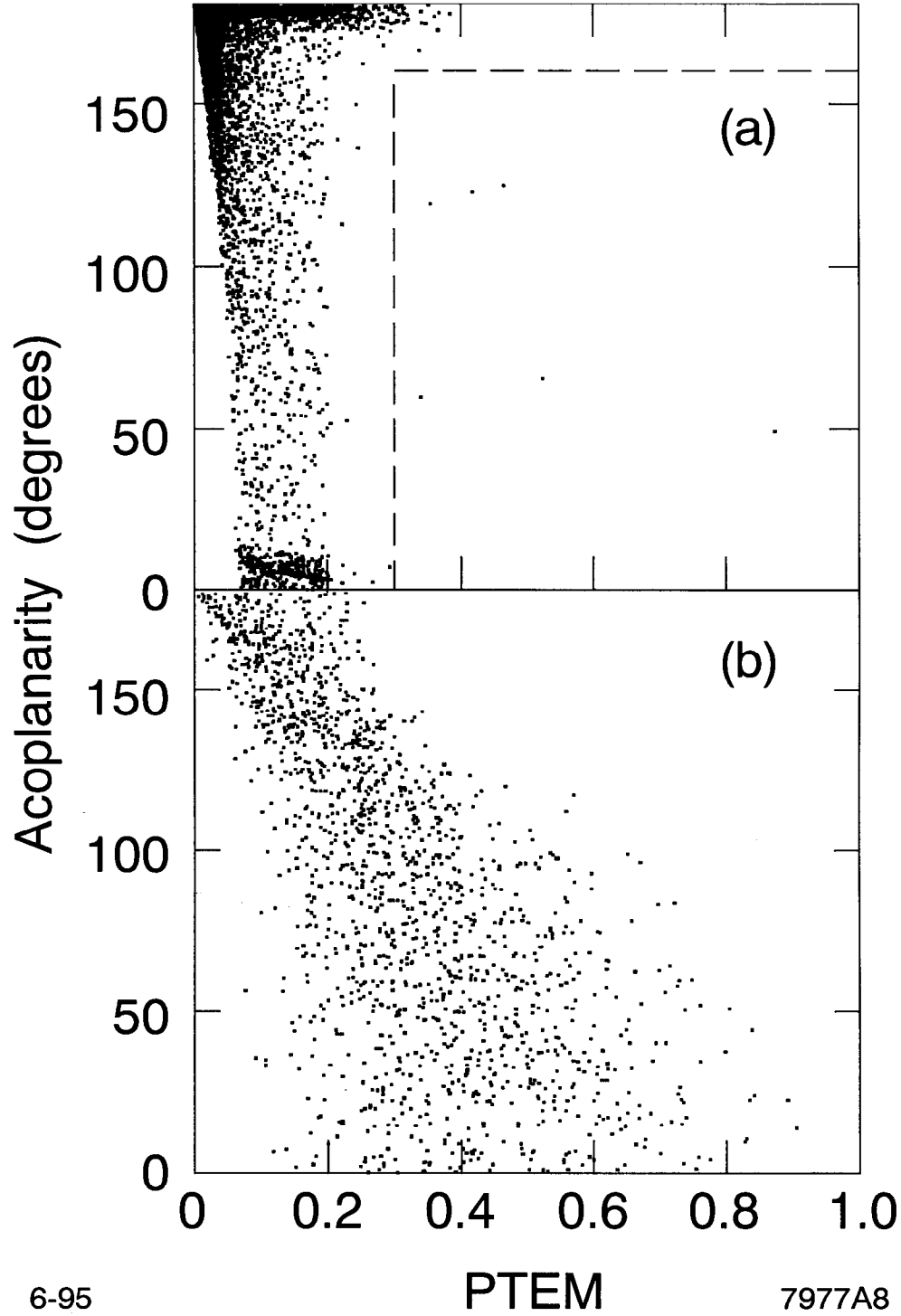
FIG. 8. (a) The scatterplot of PTEM vs. Acoplanarity for the \tau^+\tau^- candidate ee events; the dashed lines denote the region PTEM \geq 0.3 and acoplanarity \leq 160^\circ , within which events are retained. (b) The same scatterplot for ee events obtained from the \tau^+\tau^- Monte Carlo simulation after the application of the same selection criteria.
