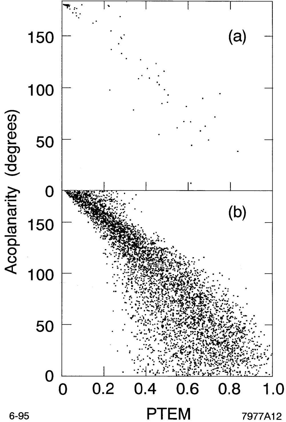
FIG. 12. (a) The scatterplot of PTEM vs. Acoplanarity for the \tau^+\tau^- candidate eh , \mu h and hh events. (b) The same scatterplot for the combined eh , \mu h and hh events obtained from the \tau^+\tau^- Monte Carlo simulation after the application of the same selection criteria.
