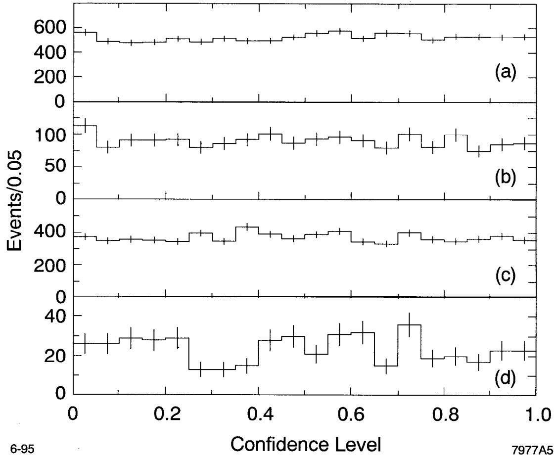
FIG. 5. The confidence level distributions for samples of a) pions from J/\psi \rightarrow \omega\pi\pi events and beam-gas electroproduction events, b) electrons from radiative Bhabha events, c) muons from \mu pair production, and d) muons from radiative \mu pair production.
