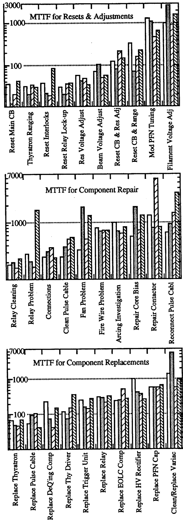
Figure 1. MTTF plots for the 244 modulator system.
