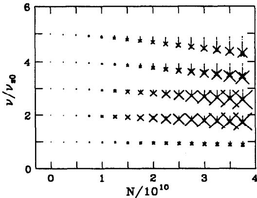
Fig. 7. Modes obtained by the Vlasov method.
