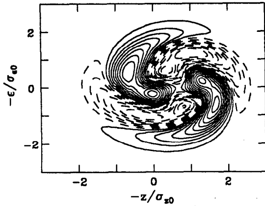
Fig. 6. Mode shape at N = 2 \times 10^{10} .
