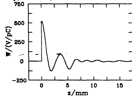
Fig. 1. The wakefield used for the simulations.
