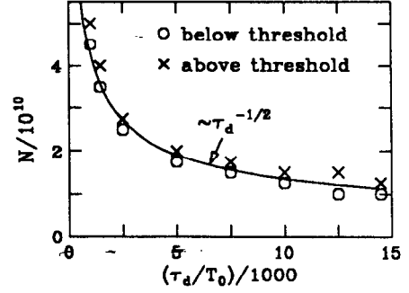
Fig. 4. N_{th} vs. \tau_d obtained by tracking.
