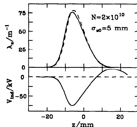
Fig. 2. A potential well example.
