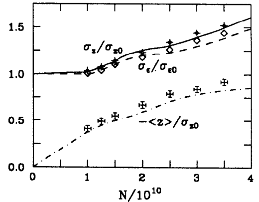
Fig. 5. Average bunch properties vs N . Shown are tracking results (plotting symbols) and the Vlasov method results (curves).
