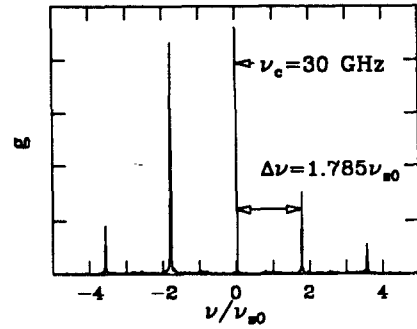
Fig. 8. Spectrum for N = 4 \times 10^{10} , \tau_d/T_0 = 1450 .
