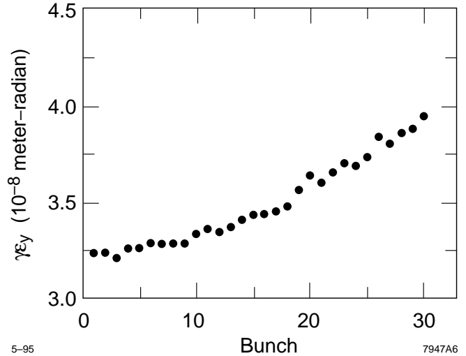
Figure 3. Simulation of emittance correction in the NLC-I pre-linac with a shortened bunch train of 30 bunches and a vacuum pressure of 3 \times 10^{-8} Torr of CO gas; because the ions are trapped, this is equivalent to a vacuum pressure of 1 \times 10^{-8} Torr and a train of 90 bunches.
