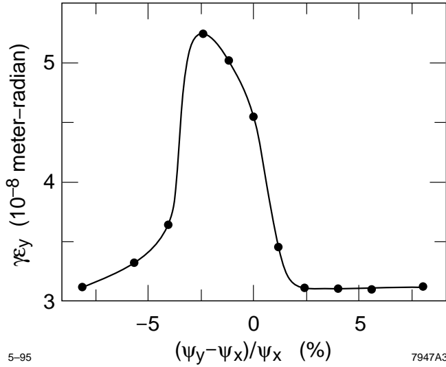
Figure 5. Emittance of the last bunch in the train versus difference between horizontal and vertical focusing in NLC-I pre-linac. This shows the effect of betatron coupling resonance; note that the resonance peak occurs for stronger horizontal focusing because of the additional vertical focusing due to the ions (from Ref. [11]).
