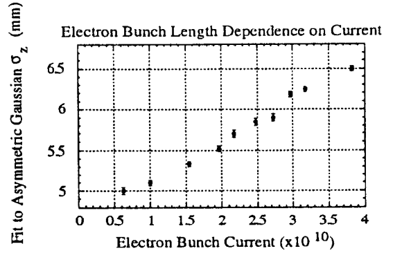
Figure 8. The bunch length dependence on current in the damping ring with V_{RF} = 820 kV.
