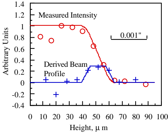
Figure 2, Measured beam profile.
