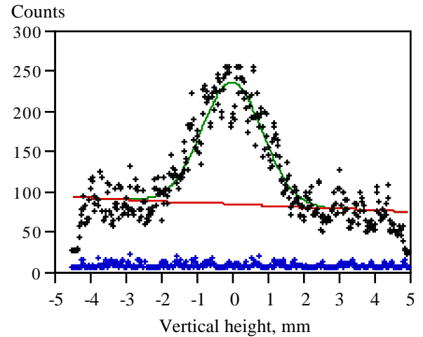
Figure 3, Vertical profile of Cherenkov Source.
