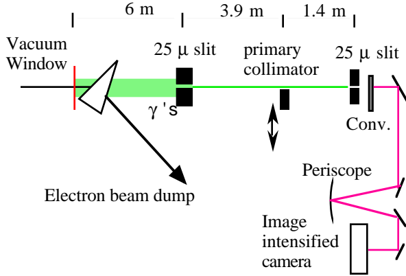
Figure 1. The experimental setup at Bates / MIT.
