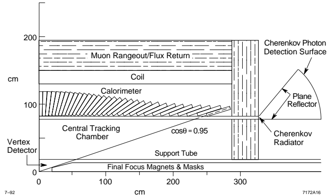
Figure 3: Schematic view of one quadrant of a model B factory detector incorporating a DIRC. The stand-off box has reflective surfaces to save PMTs.
