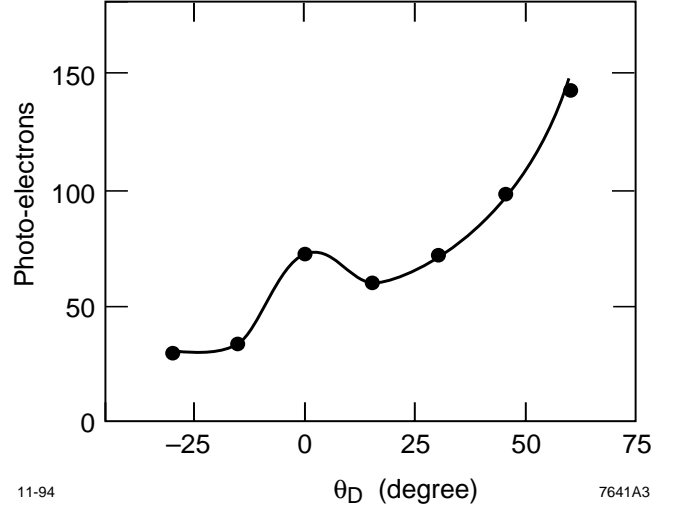
Figure 5: The observed photo-electron yield from a 1.7 cm thick bar at a track position z = 60 cm as a function of dip angle \theta_D . The solid line is a Monte-Carlo simulation. The statistical errors of the measurements are smaller than the circles. There is a scale error of 3 % due to calibration uncertainty.
