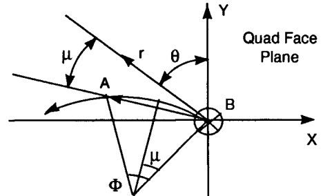
Figure 2. Mapping in solenoidal field
