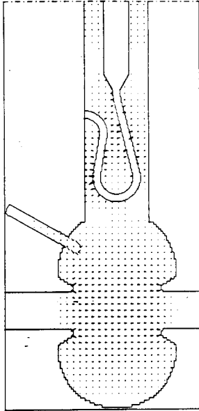
Fig. 2 Electric field of the fundamental mode with the loop coupler.
