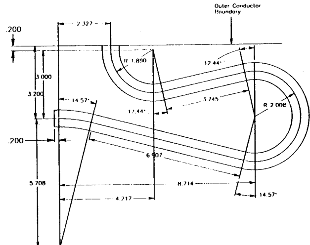
Fig. 1 The layout of the loop coupler.
