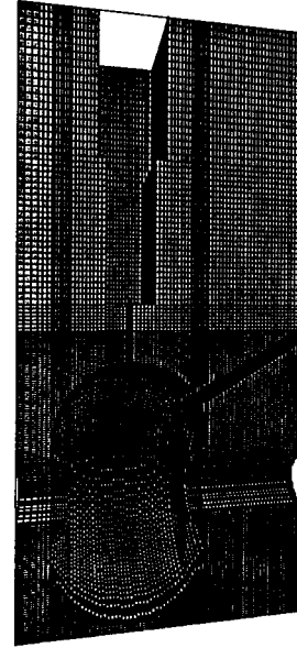
Fig. 3 MAFIA mesh for the iris coupler.
