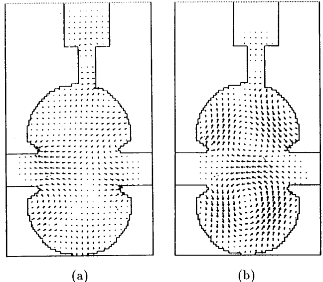
Fig. 5 Electric field pattern (a) dominated by TM_{021} mode at early times; (b) taken over by higher order TM mode at later times.
