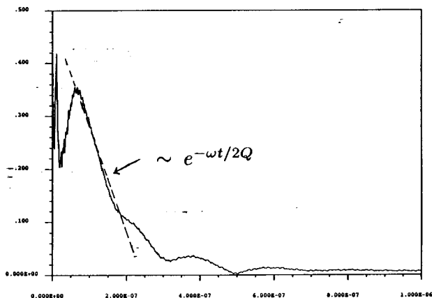
Fig. 4 Time dependence of the transmitted TE_{01} mode in the waveguide for a preloaded TM_{021} mode in the cavity. Q is determined by fitting the appropriate portion of the curve to an exponential as shown.
