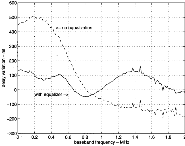
Fig. 5. Baseband group delay before and after equalization
