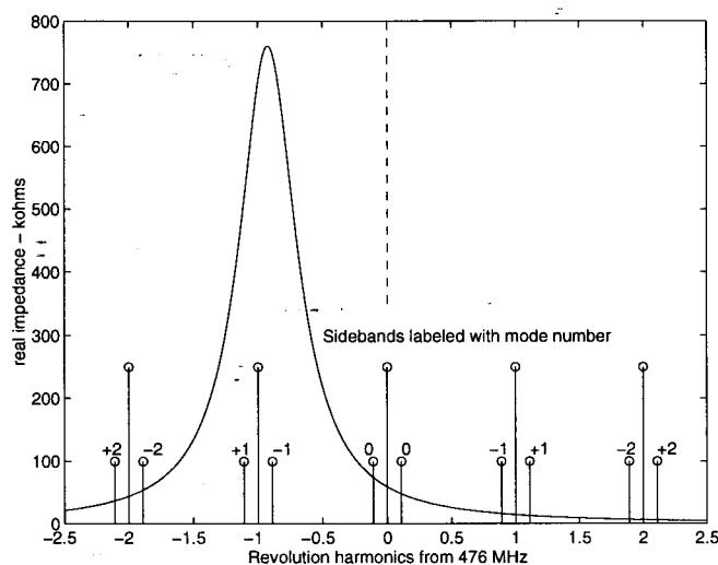
Fig. 1. Cavity impedance, revolution harmonics with sidebands
