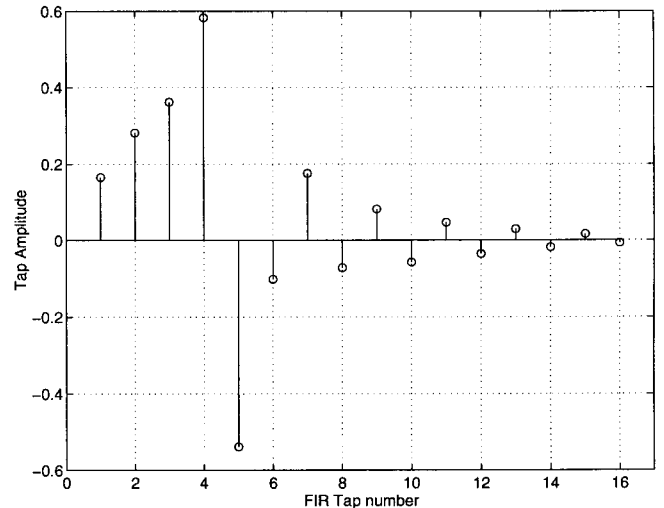
Fig. 4. Group delay equalizer tap weights used
