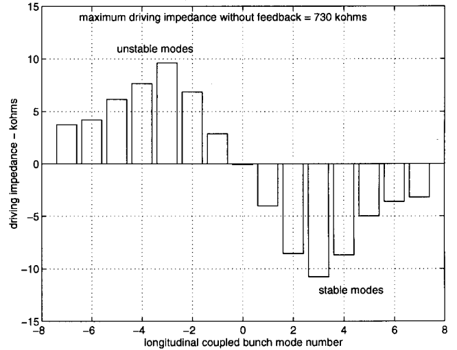
Fig. 8. Measured driving impedances for longitudinal modes -7 to +7
