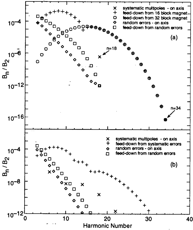
Figure 1. (a) Systematic and random harmonics for a 16-block and 32-block design. Systematic multipoles are at n=18 and 34. (b) Harmonics of a SC two-wedge design. In both plots, the feed-down harmonics result from the large offset of the LEB as it exits Q1.
