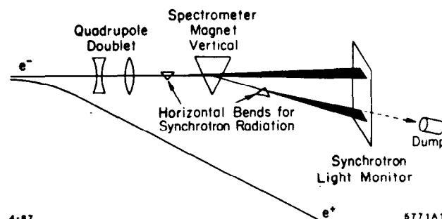
Fig. 1. Conceptual design of the extraction-line spectrometers.
