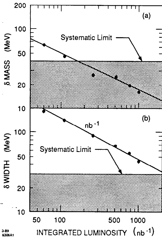
Fig. 3. Statistical errors in measuring the mass and width of the Z^0 .
