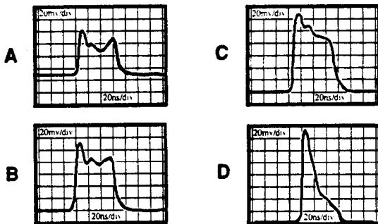
FIG. 4. RF pulse shortening observed in SHARK tests.
