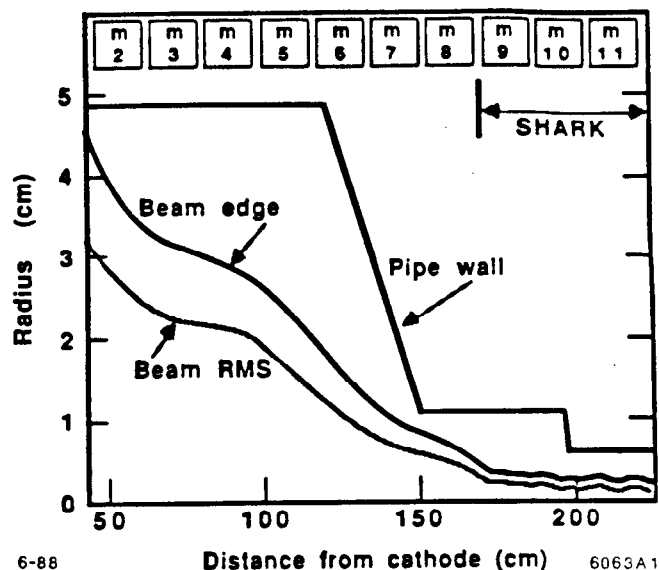
FIG. 1. Beam size calculated through SHARK.
