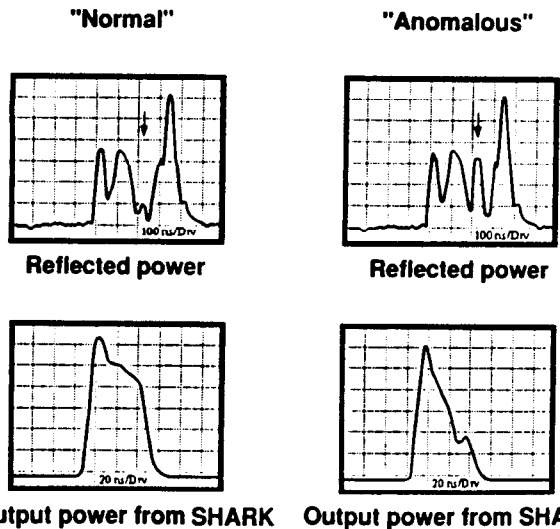
FIG. 6. SHARK reflected drive and output power. Arrows indicate the 50 nsec beam time in the reflected power.
