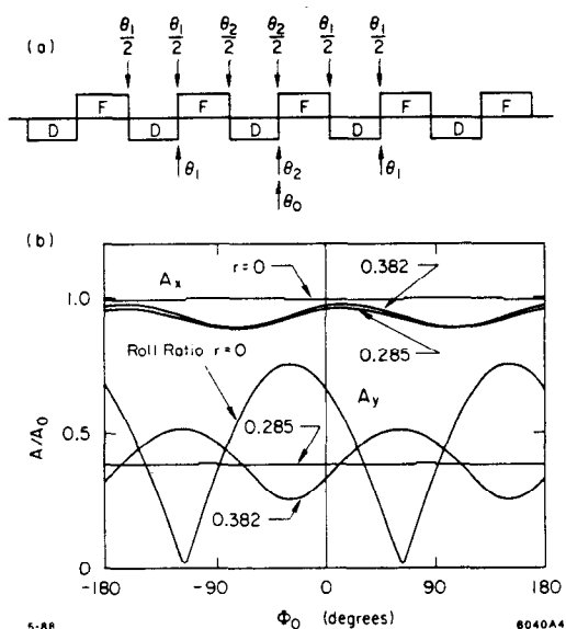
Fig. 4. (a) Typical redistribution of roll angles. (b) Cross coupling versus \Phi_0 for various values of r .
