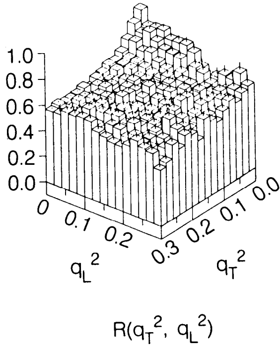
Fig. 10. The ratio of like to unlike pairs (no corrections) in the SPEAR J/\psi data. The variables q_T^2 , q_L^2 , and q_0^2 , are defined with respect to the Kopylov axis, and all variables are given in GeV^2 .
