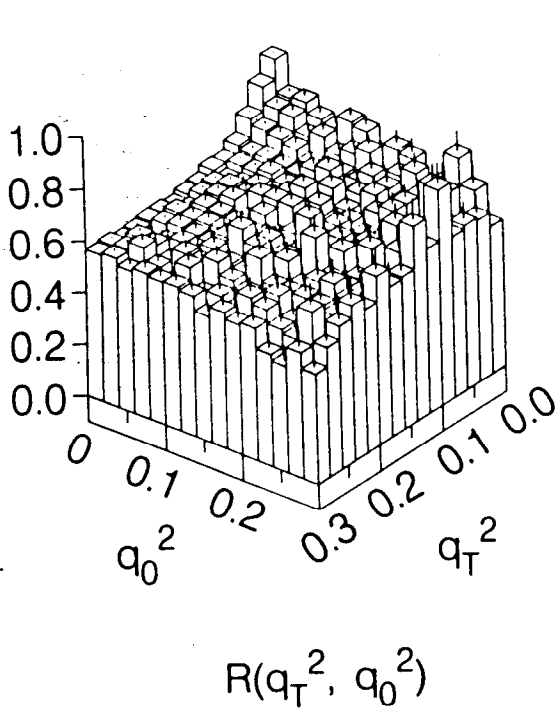
Fig. 10. The ratio of like to unlike pairs (no corrections) in the SPEAR J/\psi data. The variables q_T^2 , q_L^2 , and q_0^2 , are defined with respect to the Kopylov axis, and all variables are given in GeV^2 .
