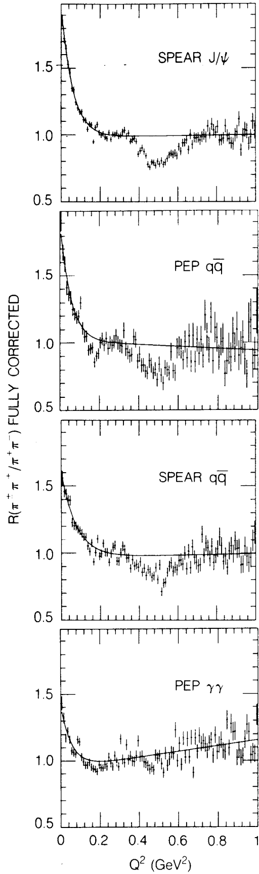
Fig. 7. Ratio of fully corrected like to unlike charged pair distributions and the fitted curves.
