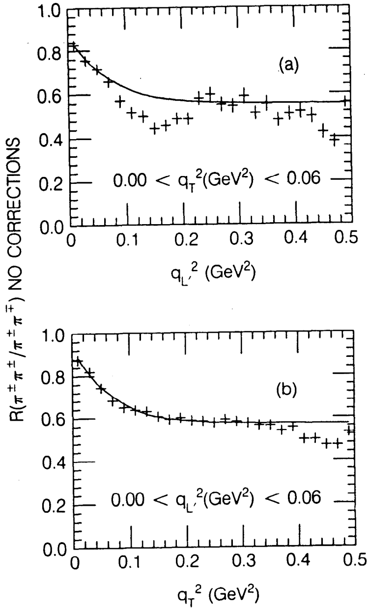
Fig. 12. The Bose-Einstein enhancement in slices of R(q_T^2, q_L^2) for the uncorrected ratio of like to unlike pairs in the SPEAR J/\psi data set. The dips due to the K^0 and \rho^0 in the unlike pairs are clearly evident in (a) the slice consisting of 0.00\text{GeV}^2 < q_T^2 < 0.06\text{ GeV}^2 projected onto the q_L^2 axis; and in (b) the slice 0.00\text{GeV}^2 < q_L^2 < 0.06\text{ GeV}^2 projected onto the q_T^2 axis.
