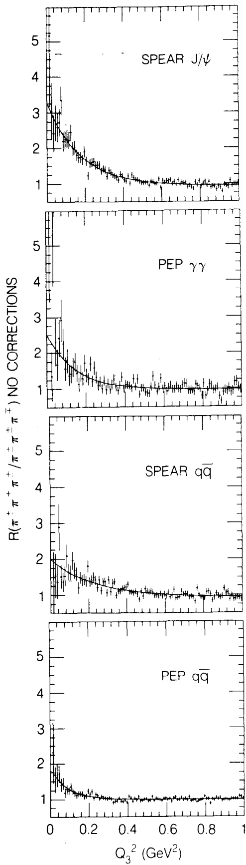
Fig. 5. Ratio of like to \pm\pm\mp triplet distributions with no corrections applied.
