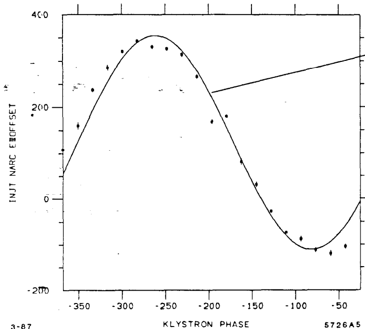
Fig. 3. Klystron phase-energy analysis.
