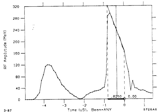
Fig. 1. SLED RF wave shape.
