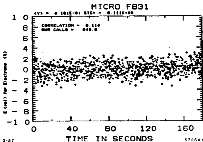
Fig. 5. Typical stable energy plot
