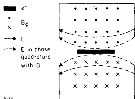
Fig. 2. Simplified field plots a) in traveling-wave accelerator showing radial RF force as electrons are being bunched and fall back on the wave; b) in standing-wave accelerator.
