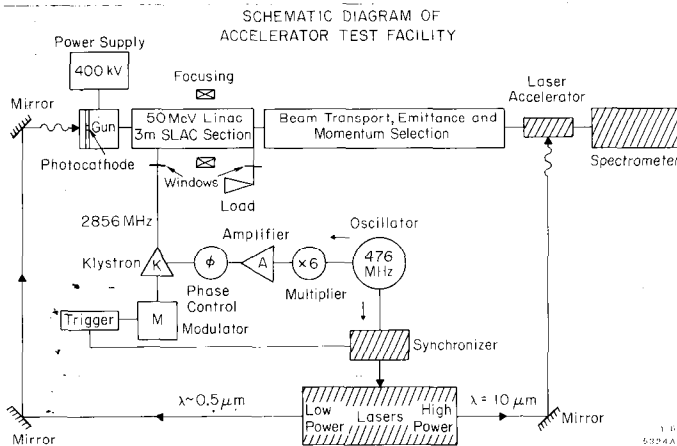
Fig. 1. Schematic diagram of Accelerator Test Facility.
