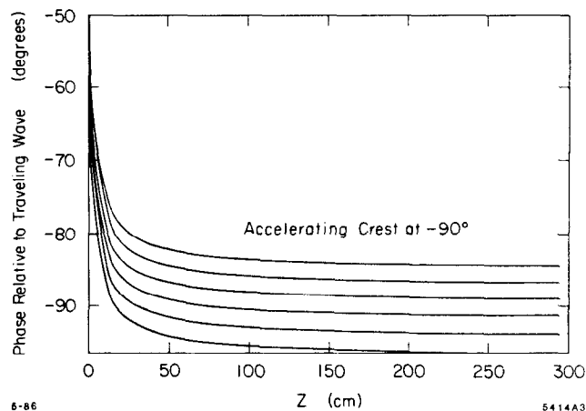
Fig. 5. Longitudinal orbits: phase versus z position.
