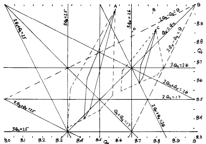
Fig. 3 - AGS tune space.
