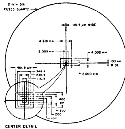
Fig. 2 -- Reticle Design Two-Power Magnification
