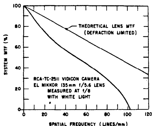
Fig. 4 -- High-Power Modulation Transfer Function
