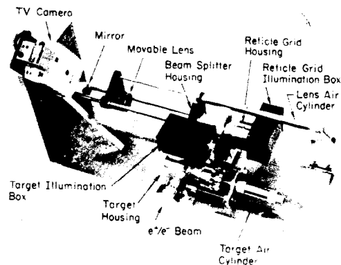
Fig. 3 -- Profile Monitor Assembly
