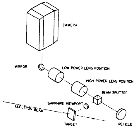
Fig. 1 -- Optical Arrangement of Profile Monitor
