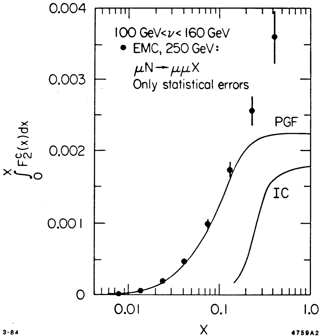
Fig. 2. EMC data 12 for the integrated charm quark x_{Bj} distribution in the nucleon deduced from \mu N \rightarrow \mu \mu X . The photon-gluon fusion (PGF) model predicts that the integrated momentum distribution saturates at x_{Bj} = 0.1 whereas the data indicates a substantial contribution beyond x_{Bj} = 0.4 . The intrinsic charm (IC) prediction is from Ref. 15.
