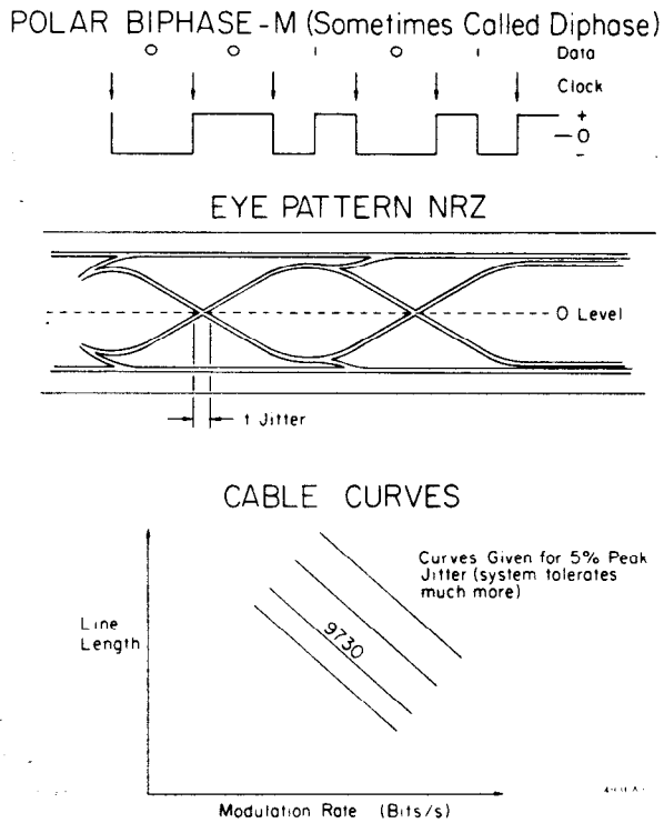
Figure 5. Line Signals.
