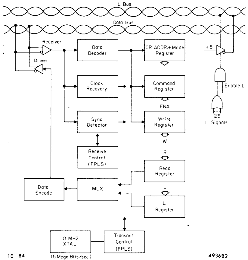
Figure 4. Serial Crate Controller-Block Diagram.
