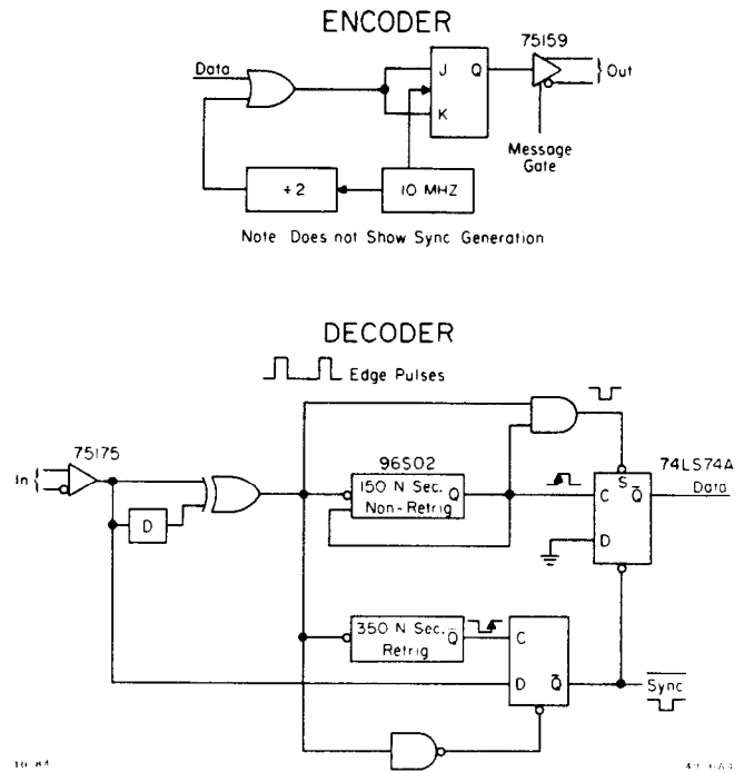
Figure 6. Encoder/Decoder Circuits.
