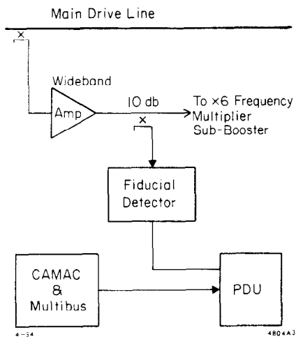
Fig. 4. Fiducial pickoff.
