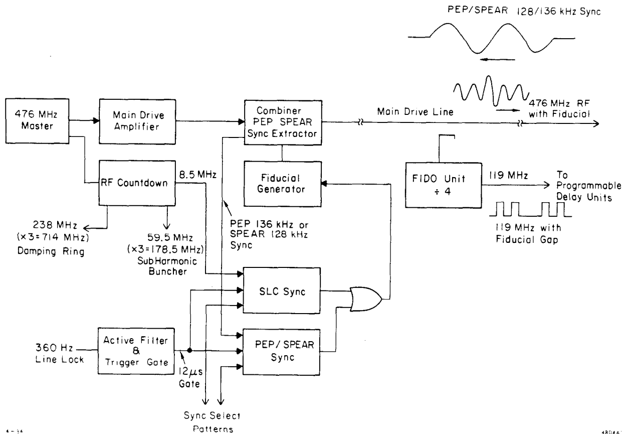
Fig. 1. Block Diagram of the driveline based trigger system.
