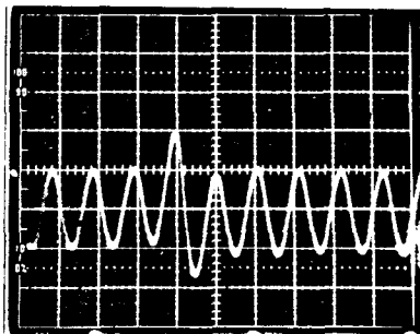
Fig. 2. Fiducial on 476 MHz (2 nsec/cm).
