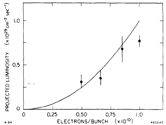
Fig. 5. Projected luminosity based on beam measurements taken during the January 1984 tests.
