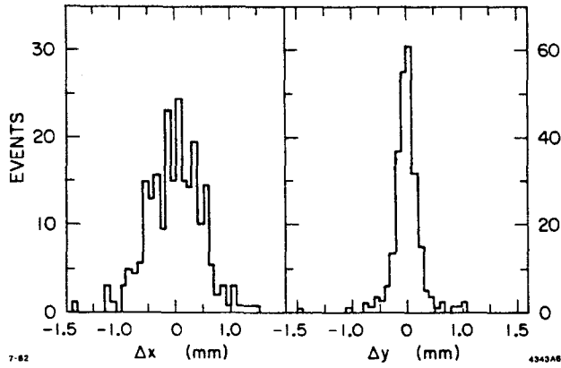
Fig. 1 : Horizontal and vertical hadronic vertex positions relative to the beam position. Only those runs with tau decays are shown.
