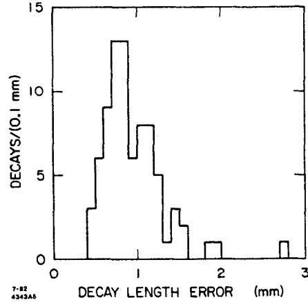
Fig. 2 : Calculated error in the decay length.
