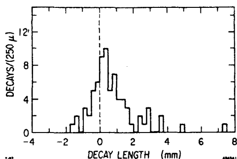
Fig. 3 : Measured decay lengths.
